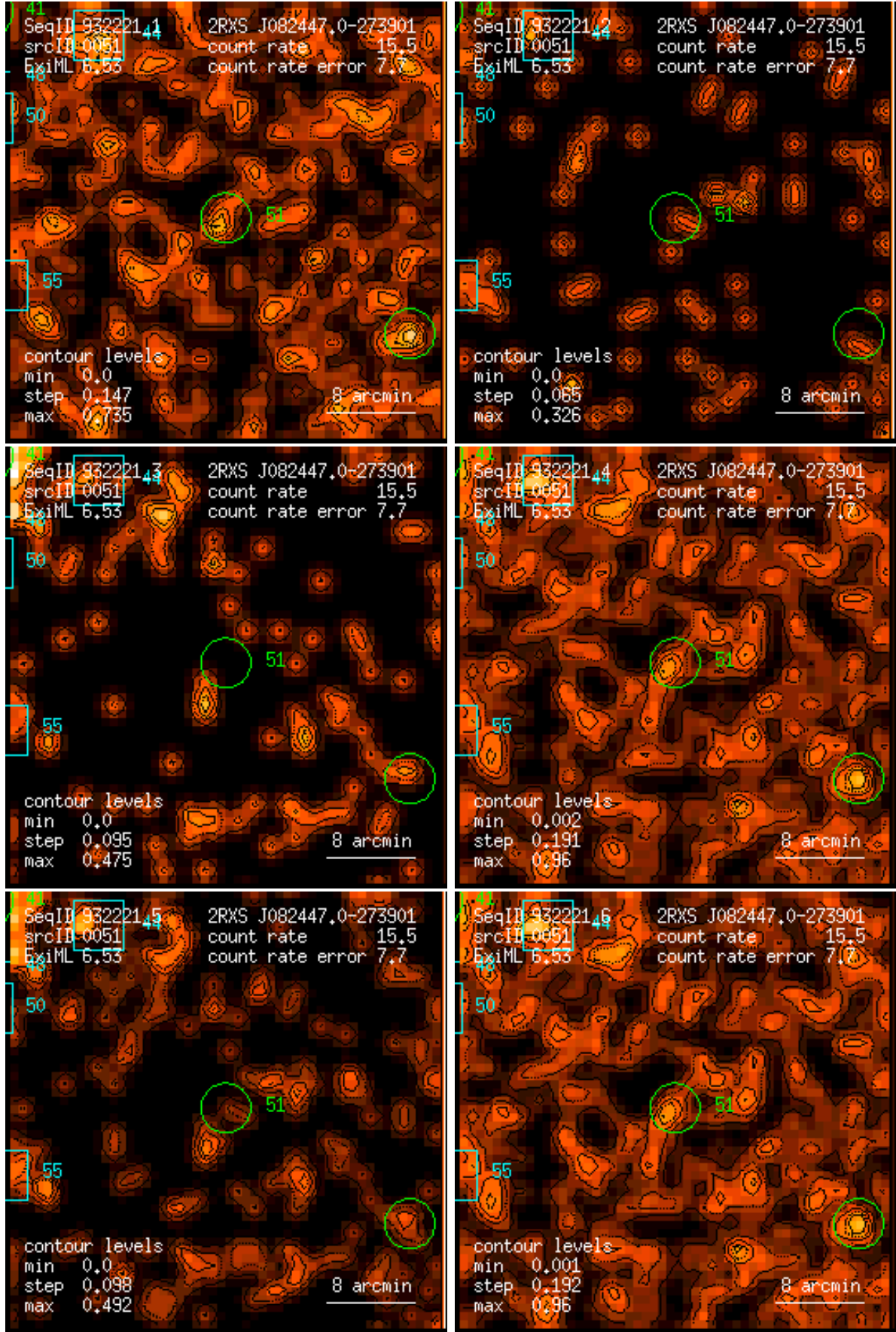
Figure 51: RASS 932221: detection 0051: band rate images, Gaussian filter: (1) PSPC channels 11 – 41, (2) 52 – 90, (3) 91 – 201, (4) 11 – 235, (5) 52 – 201, (6) 11 – 201. Broad band rates in counts/ks. Band rate contour levels in counts/ks/arcmin 2 .
