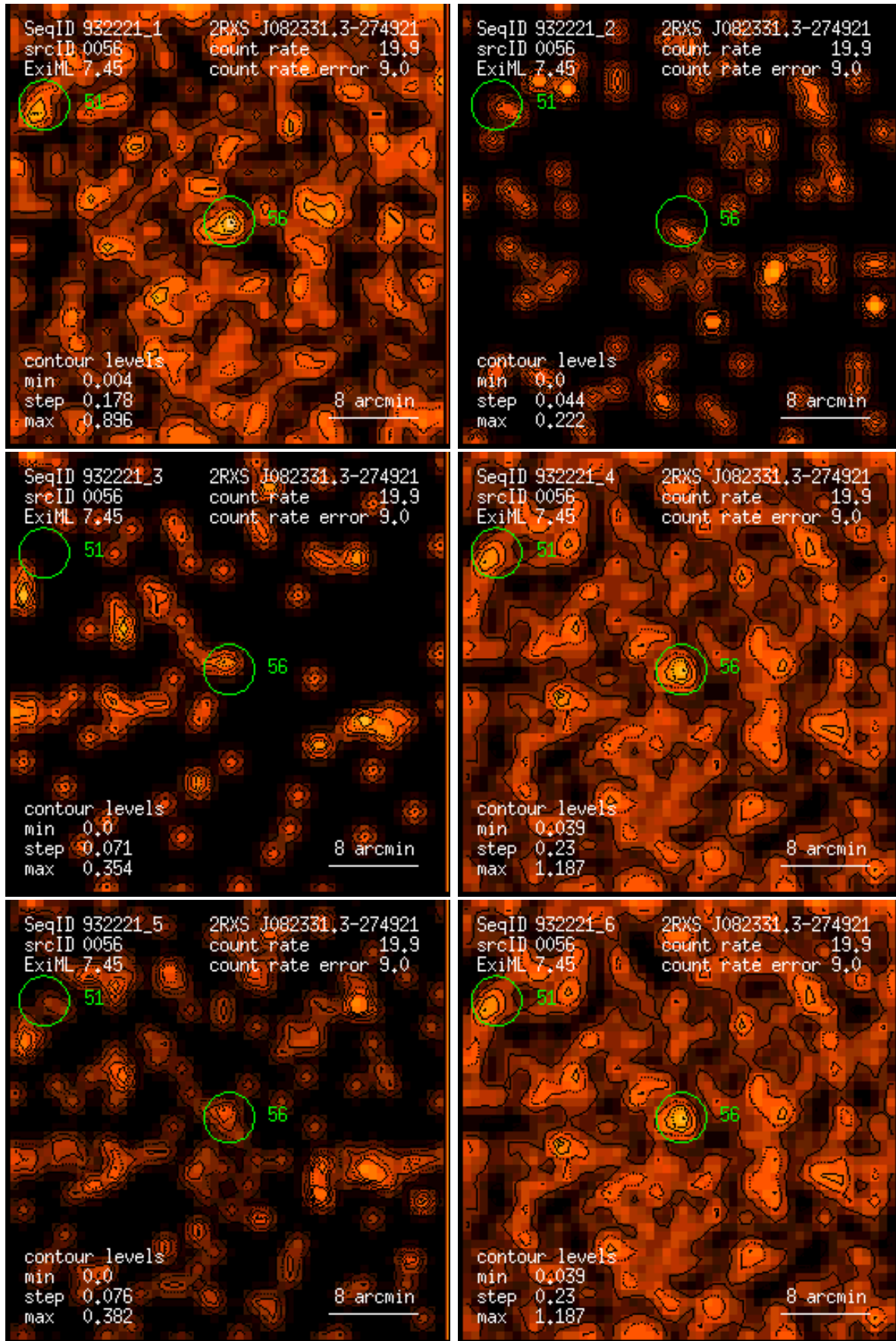
Figure 56: RASS 932221: detection 0056: band rate images, Gaussian filter: (1) PSPC channels 11 – 41, (2) 52 – 90, (3) 91 – 201, (4) 11 – 235, (5) 52 – 201, (6) 11 – 201. Broad band rates in counts/ks. Band rate contour levels in counts/ks/arcmin 2 .
