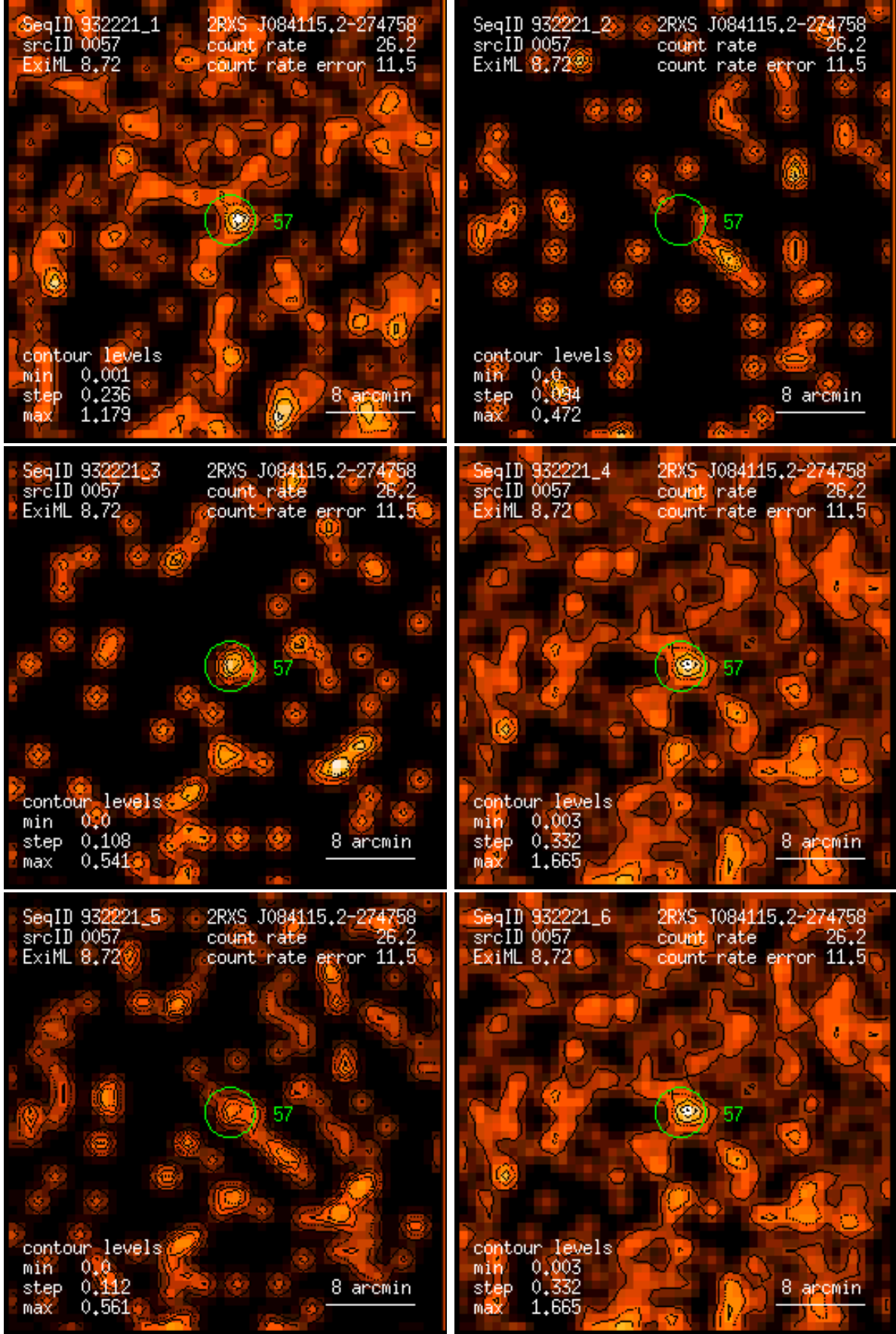
Figure 57: RASS 932221: detection 0057: band rate images, Gaussian filter: (1) PSPC channels 11 – 41, (2) 52 – 90, (3) 91 – 201, (4) 11 – 235, (5) 52 – 201, (6) 11 – 201. Broad band rates in counts/ks. Band rate contour levels in counts/ks/arcmin 2 .
