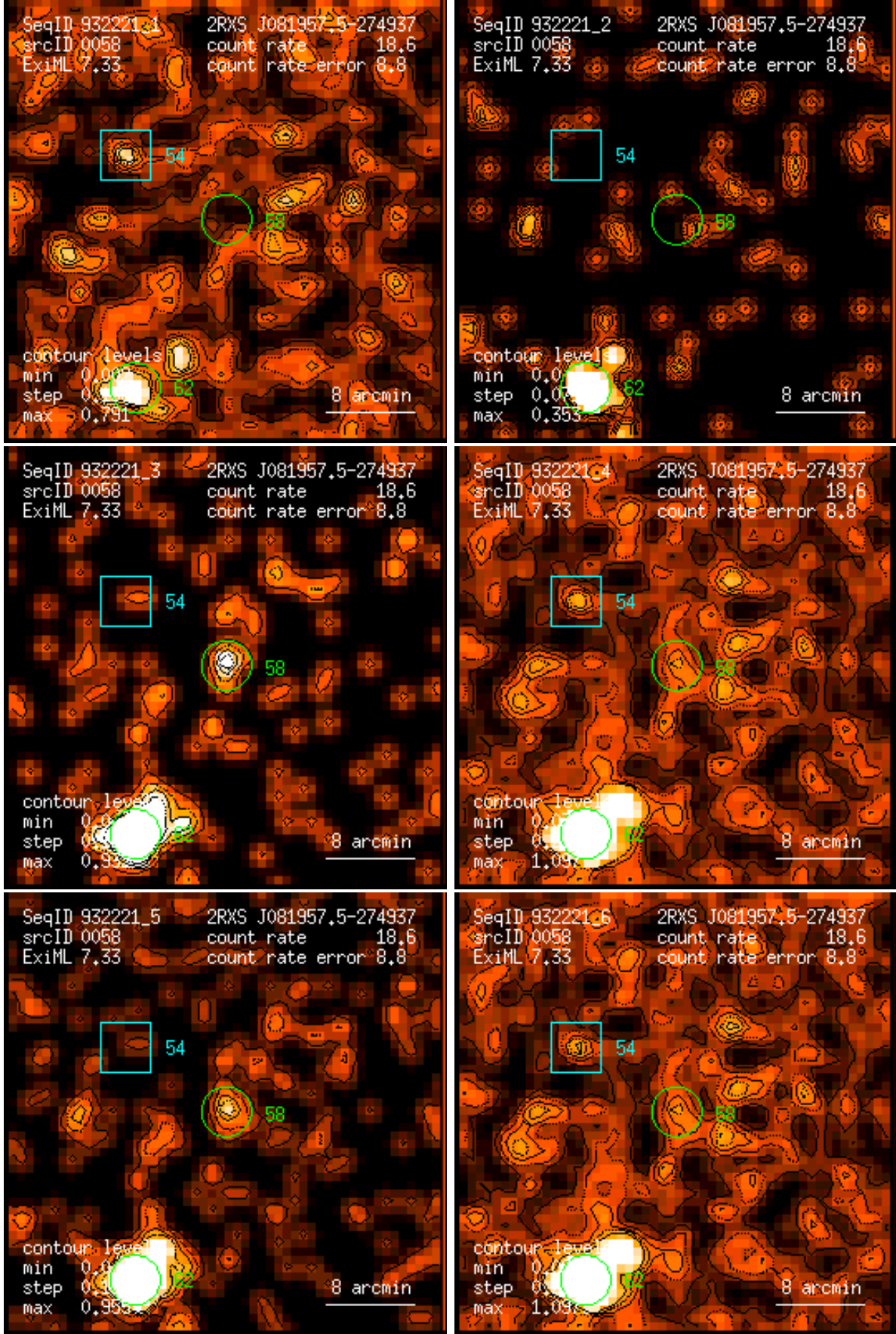
Figure 58: RASS 932221: detection 0058: band rate images, Gaussian filter: (1) PSPC channels 11 – 41, (2) 52 – 90, (3) 91 – 201, (4) 11 – 235, (5) 52 – 201, (6) 11 – 201. Broad band rates in counts/ks. Band rate contour levels in counts/ks/arcmin 2 .
