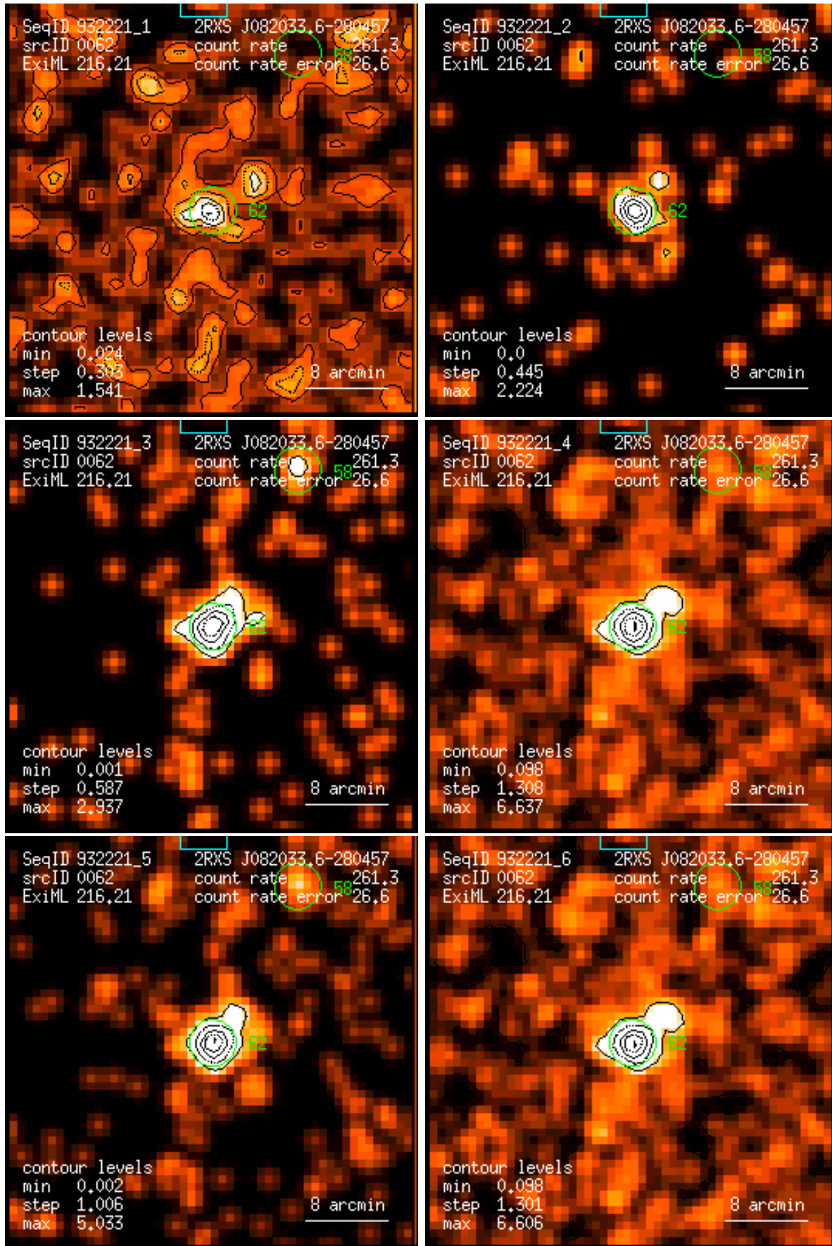
Figure 62: RASS 932221: detection 0062: band rate images, Gaussian filter: (1) PSPC channels 11 – 41, (2) 52 – 90, (3) 91 – 201, (4) 11 – 235, (5) 52 – 201, (6) 11 – 201. Broad band rates in counts/ks. Band rate contour levels in counts/ks/arcmin 2 .
