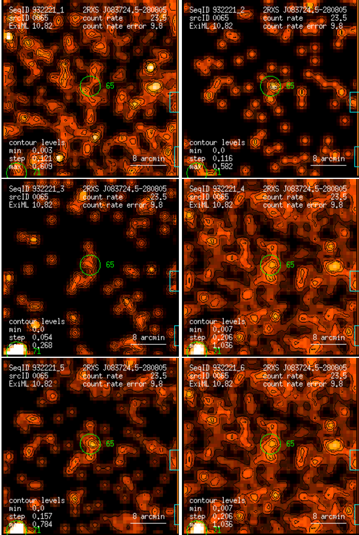
Figure 65: RASS 932221: detection 0065: band rate images, Gaussian filter: (1) PSPC channels 11 – 41, (2) 52 – 90, (3) 91 – 201, (4) 11 – 235, (5) 52 – 201, (6) 11 – 201. Broad band rates in counts/ks. Band rate contour levels in counts/ks/arcmin 2 .
