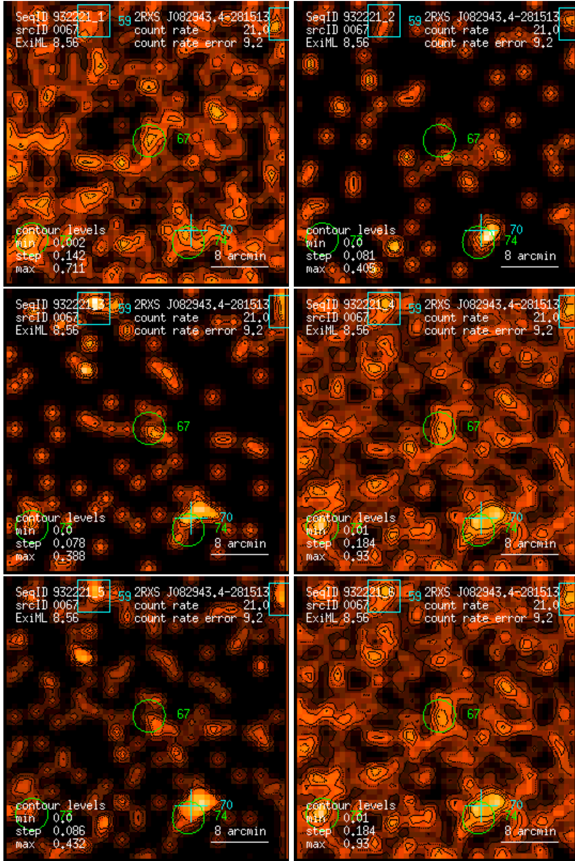
Figure 67: RASS 932221: detection 0067: band rate images, Gaussian filter: (1) PSPC channels 11 – 41, (2) 52 – 90, (3) 91 – 201, (4) 11 – 235, (5) 52 – 201, (6) 11 – 201. Broad band rates in counts/ks. Band rate contour levels in counts/ks/arcmin 2 .
