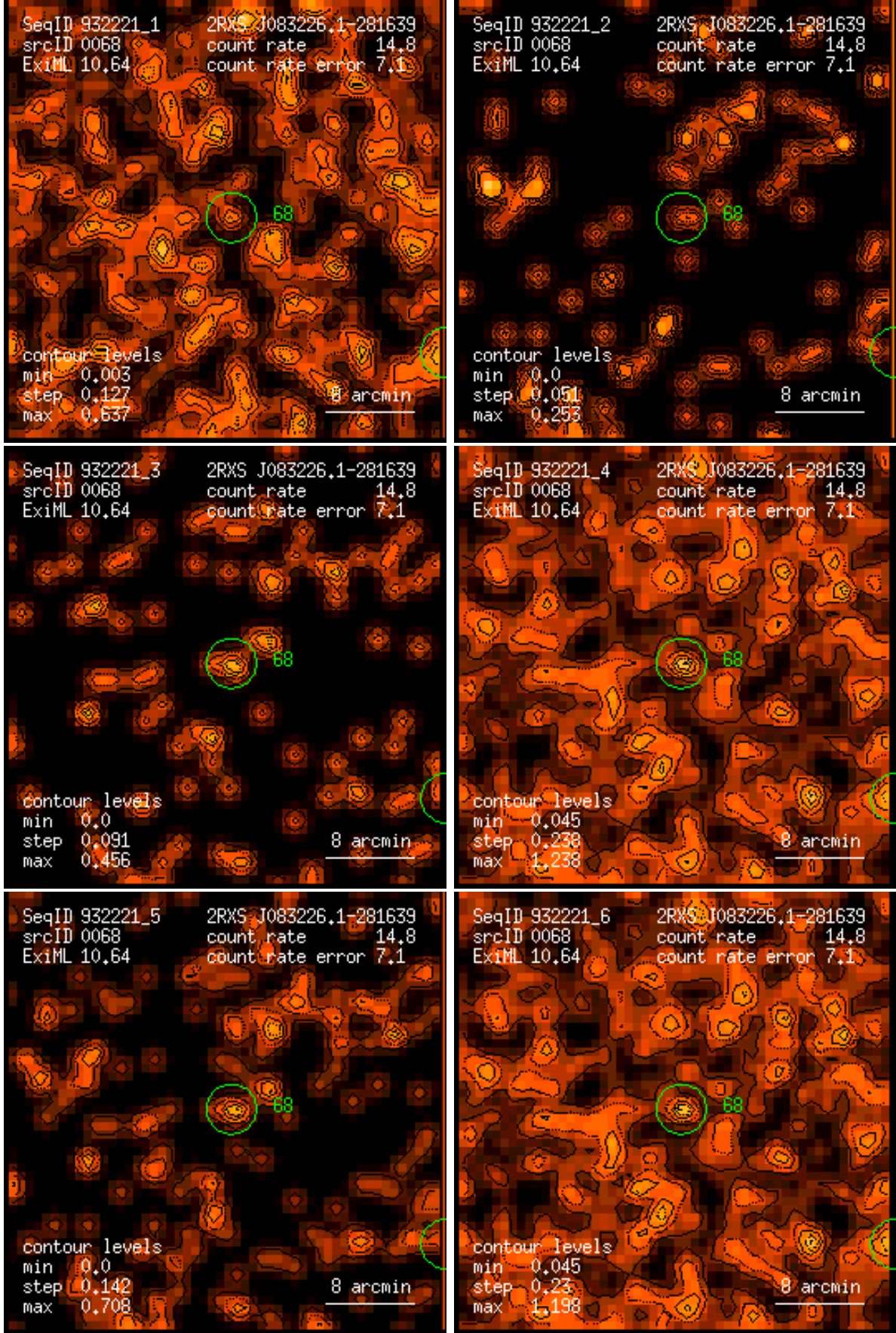
Figure 68: RASS 932221: detection 0068: band rate images, Gaussian filter: (1) PSPC channels 11 – 41, (2) 52 – 90, (3) 91 – 201, (4) 11 – 235, (5) 52 – 201, (6) 11 – 201. Broad band rates in counts/ks. Band rate contour levels in counts/ks/arcmin 2 .
