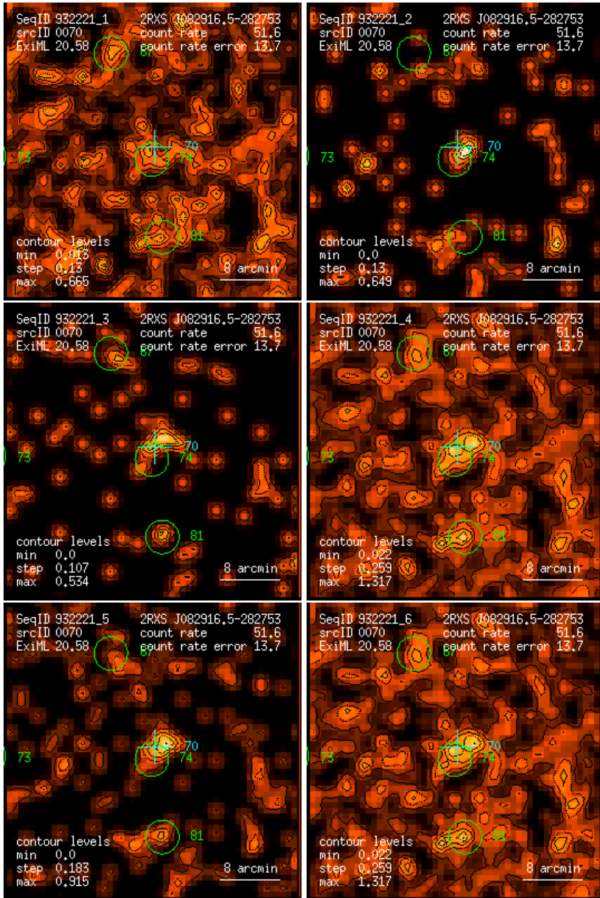
Figure 70: RASS 932221: detection 0070: band rate images, Gaussian filter: (1) PSPC channels 11 – 41, (2) 52 – 90, (3) 91 – 201, (4) 11 – 235, (5) 52 – 201, (6) 11 – 201. Broad band rates in counts/ks. Band rate contour levels in counts/ks/arcmin 2 .
