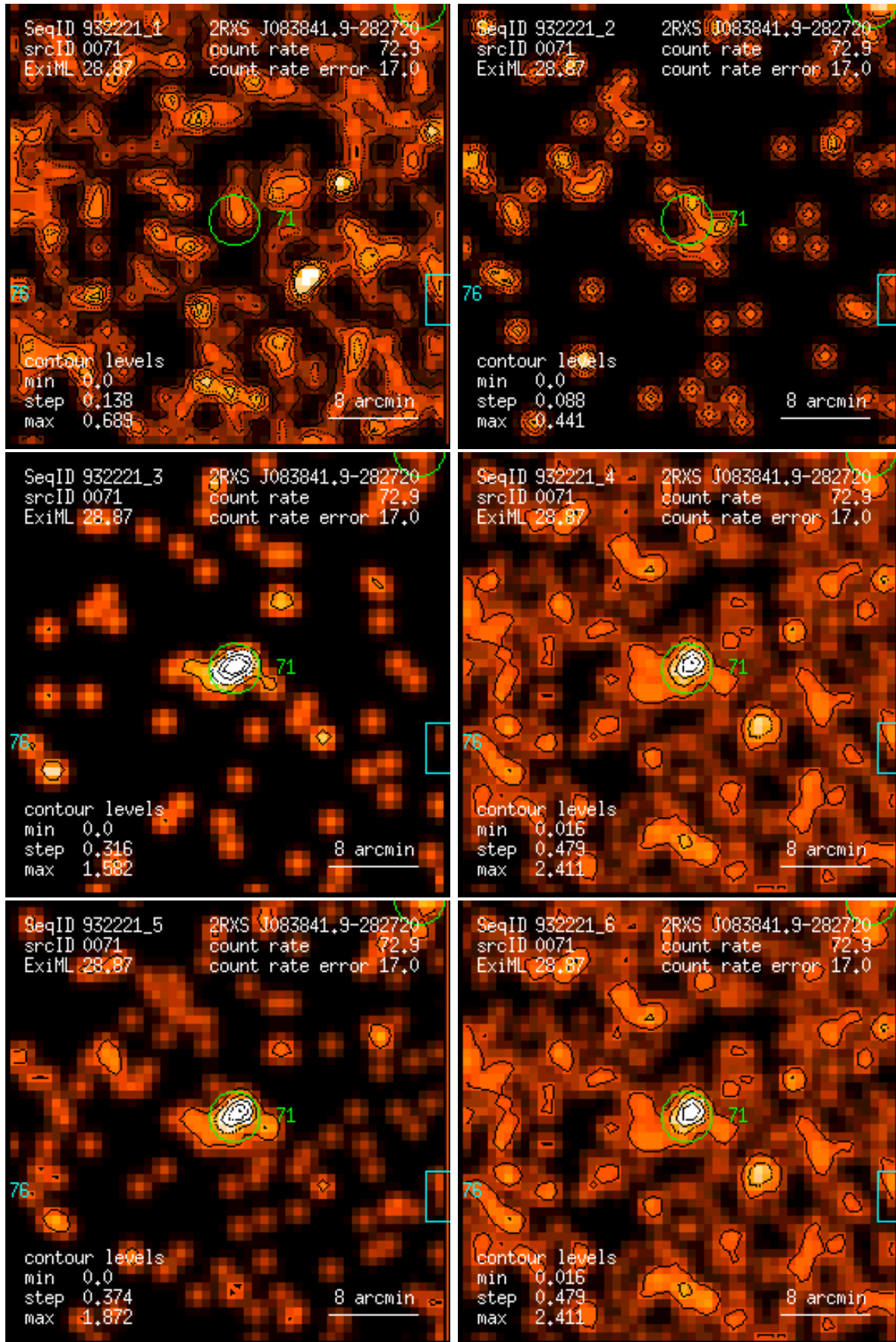
Figure 71: RASS 932221: detection 0071: band rate images, Gaussian filter: (1) PSPC channels 11 – 41, (2) 52 – 90, (3) 91 – 201, (4) 11 – 235, (5) 52 – 201, (6) 11 – 201. Broad band rates in counts/ks. Band rate contour levels in counts/ks/arcmin 2 .
