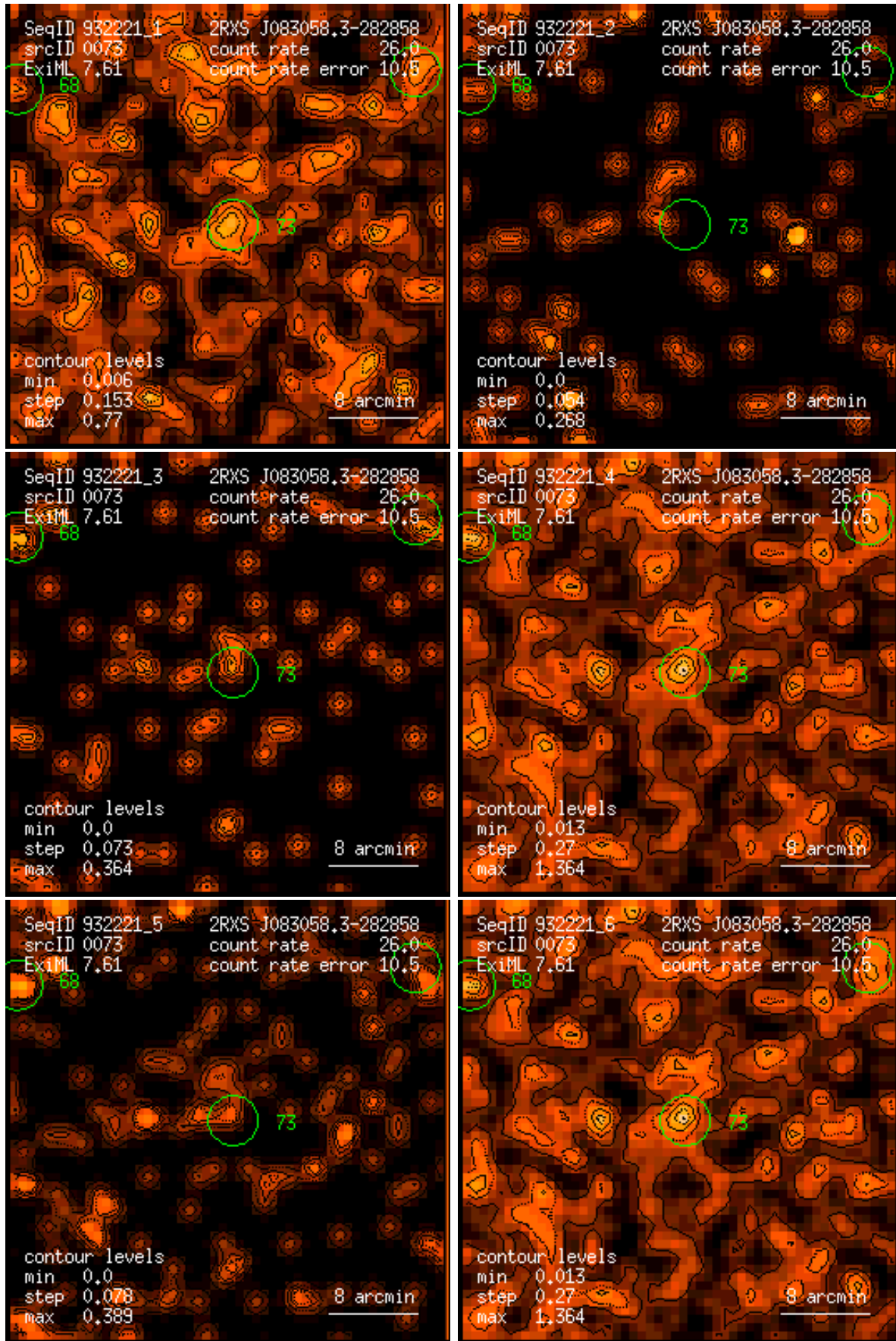
Figure 73: RASS 932221: detection 0073: band rate images, Gaussian filter: (1) PSPC channels 11 – 41, (2) 52 – 90, (3) 91 – 201, (4) 11 – 235, (5) 52 – 201, (6) 11 – 201. Broad band rates in counts/ks. Band rate contour levels in counts/ks/arcmin 2 .
