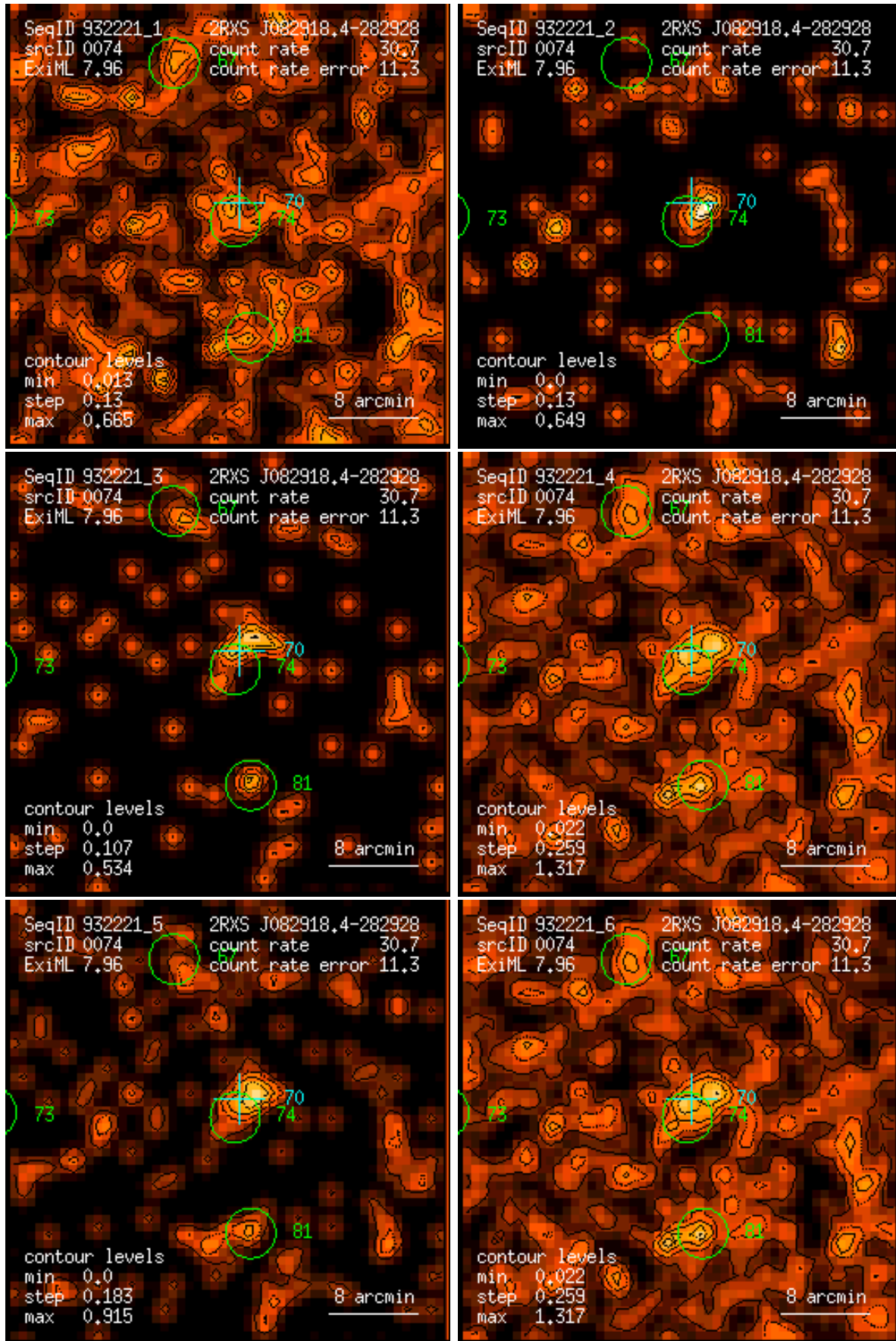
Figure 74: RASS 932221: detection 0074: band rate images, Gaussian filter: (1) PSPC channels 11 – 41, (2) 52 – 90, (3) 91 – 201, (4) 11 – 235, (5) 52 – 201, (6) 11 – 201. Broad band rates in counts/ks. Band rate contour levels in counts/ks/arcmin 2 .
