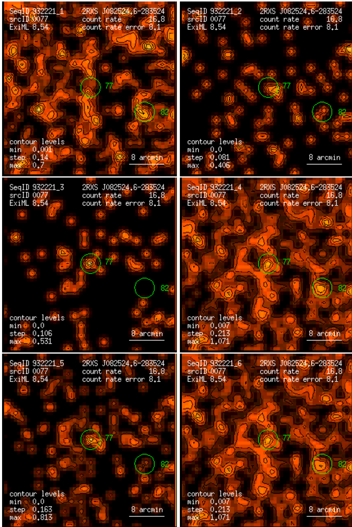
Figure 77: RASS 932221: detection 0077: band rate images, Gaussian filter: (1) PSPC channels 11 – 41, (2) 52 – 90, (3) 91 – 201, (4) 11 – 235, (5) 52 – 201, (6) 11 – 201. Broad band rates in counts/ks. Band rate contour levels in counts/ks/arcmin 2 .
