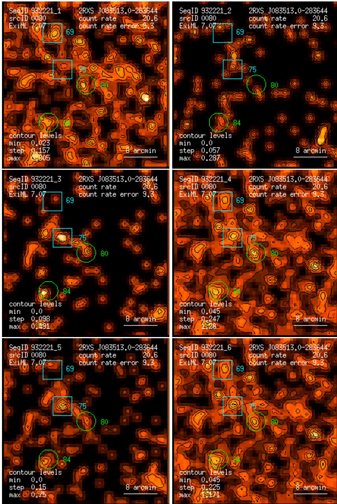
Figure 80: RASS 932221: detection 0080: band rate images, Gaussian filter: (1) PSPC channels 11 – 41, (2) 52 – 90, (3) 91 – 201, (4) 11 – 235, (5) 52 – 201, (6) 11 – 201. Broad band rates in counts/ks. Band rate contour levels in counts/ks/arcmin 2 .
