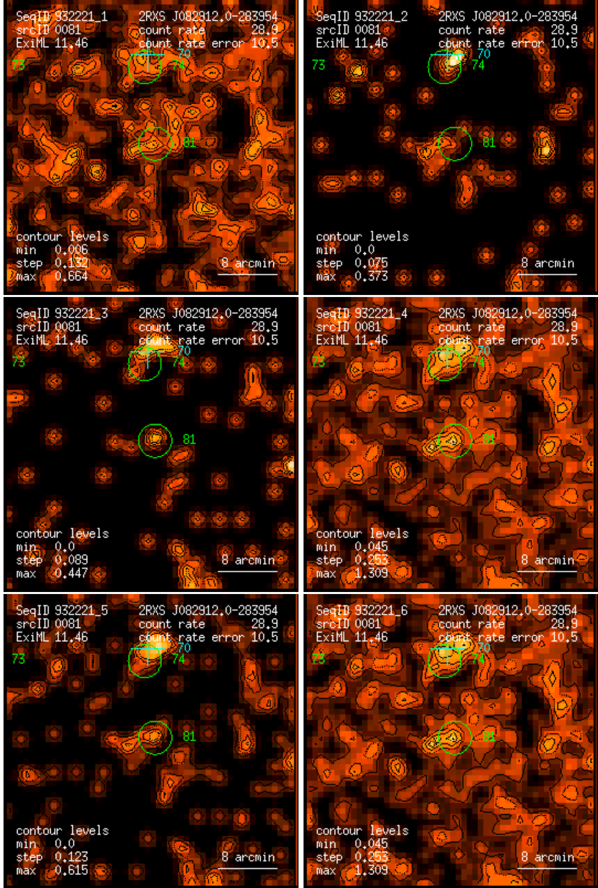
Figure 81: RASS 932221: detection 0081: band rate images, Gaussian filter: (1) PSPC channels 11 – 41, (2) 52 – 90, (3) 91 – 201, (4) 11 – 235, (5) 52 – 201, (6) 11 – 201. Broad band rates in counts/ks. Band rate contour levels in counts/ks/arcmin 2 .
