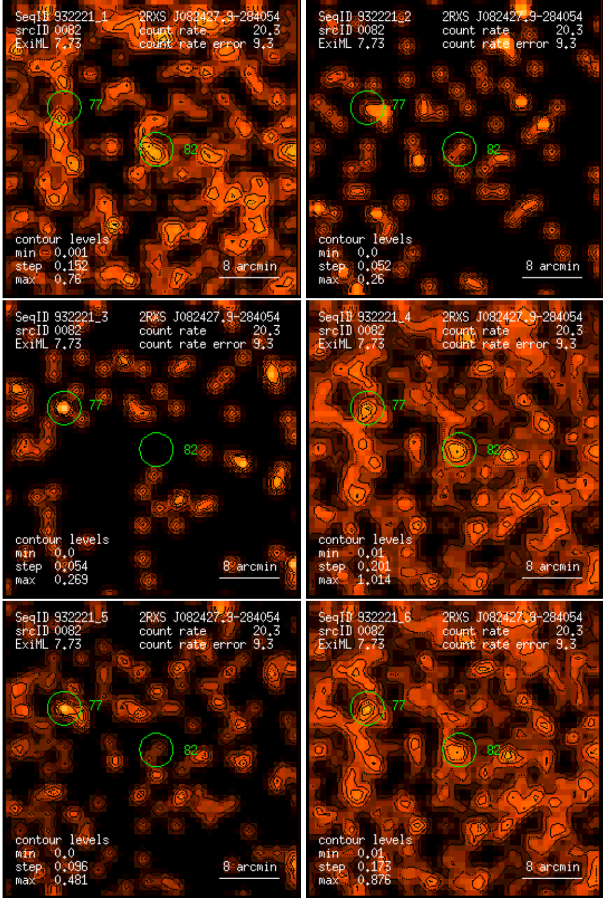
Figure 82: RASS 932221: detection 0082: band rate images, Gaussian filter: (1) PSPP channels 11 – 41, (2) 52 – 90, (3) 91 – 201, (4) 11 – 235, (5) 52 – 201, (6) 11 – 201. Broad band rates in counts/ks. Band rate contour levels in counts/ks/arcmin 2 .
