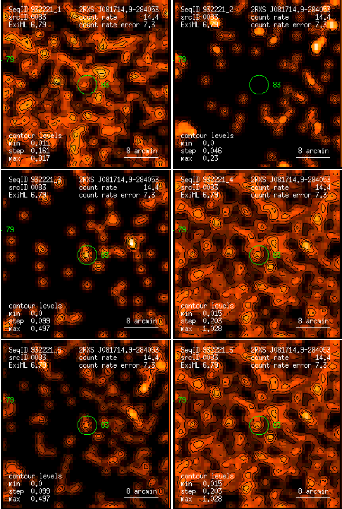
Figure 83: RASS 932221: detection 0083: band rate images, Gaussian filter: (1) PSPC channels 11 – 41, (2) 52 – 90, (3) 91 – 201, (4) 11 – 235, (5) 52 – 201, (6) 11 – 201. Broad band rates in counts/ks. Band rate contour levels in counts/ks/arcmin 2 .
