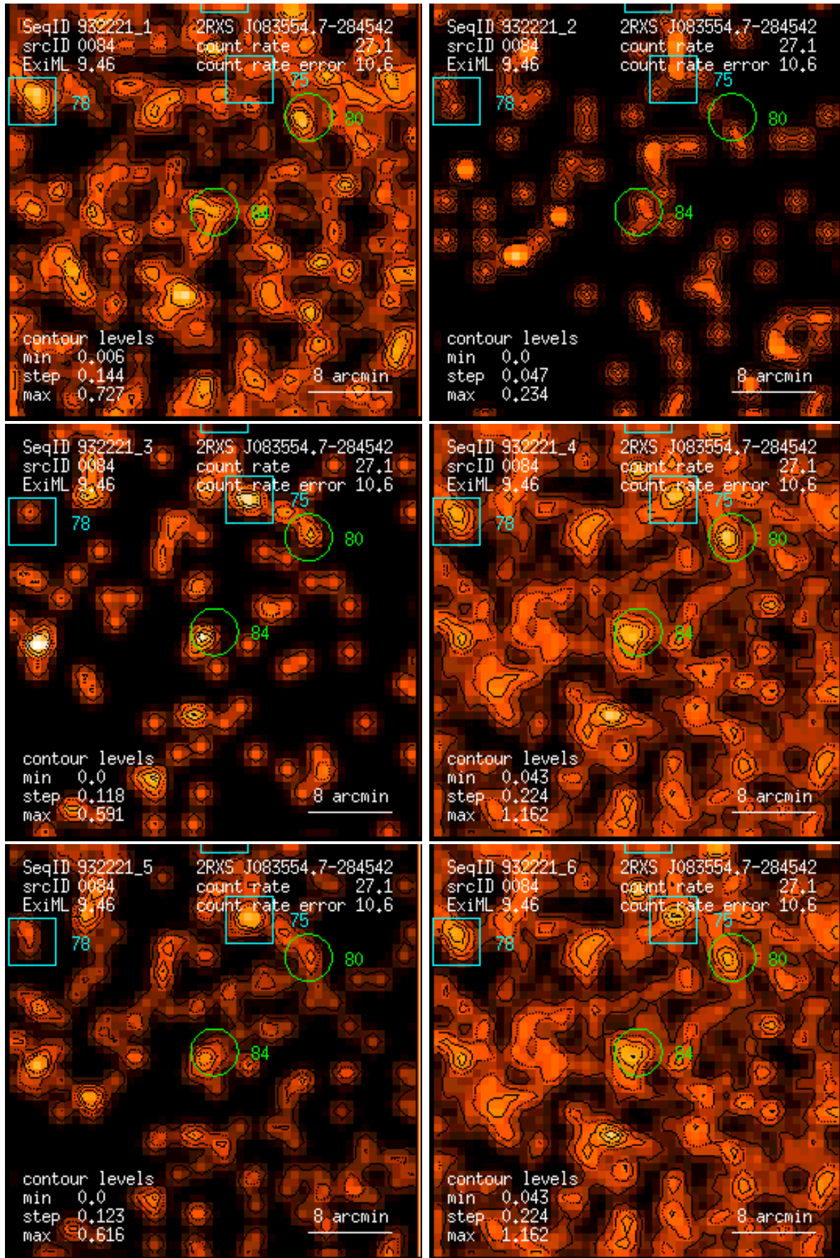
Figure 84: RASS 932221: detection 0084: band rate images, Gaussian filter: (1) PSPC channels 11 – 41, (2) 52 – 90, (3) 91 – 201, (4) 11 – 235, (5) 52 – 201, (6) 11 – 201. Broad band rates in counts/ks. Band rate contour levels in counts/ks/arcmin 2 .
