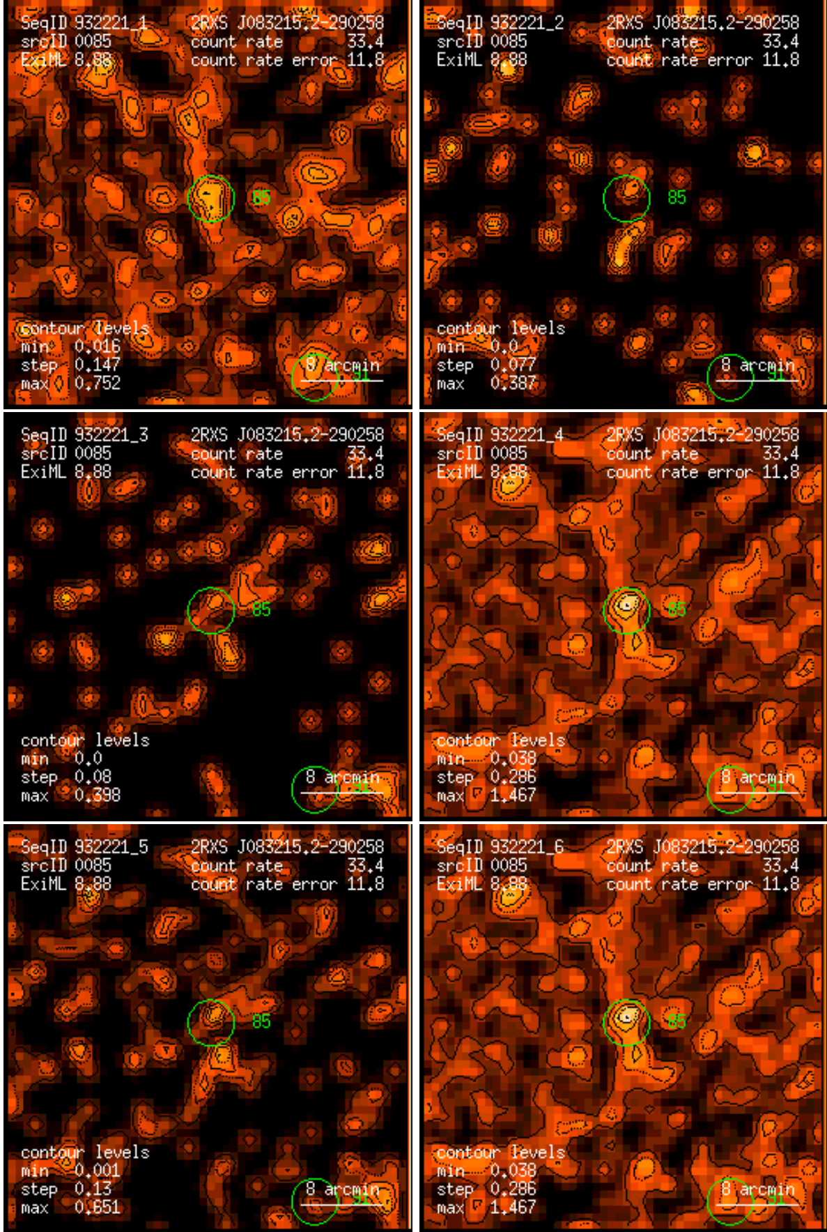
Figure 85: RASS 932221: detection 0085: band rate images, Gaussian filter: (1) PSPC channels 11 – 41, (2) 52 – 90, (3) 91 – 201, (4) 11 – 235, (5) 52 – 201, (6) 11 – 201. Broad band rates in counts/ks. Band rate contour levels in counts/ks/arcmin 2 .
