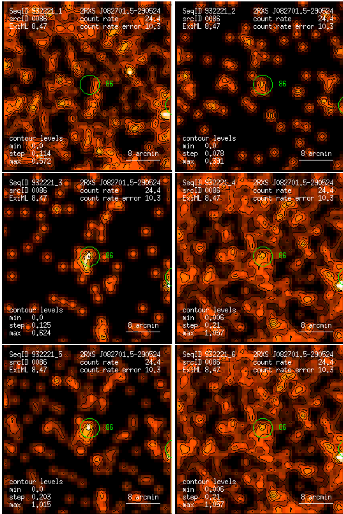
Figure 86: RASS 932221: detection 0086: band rate images, Gaussian filter: (1) PSPC channels 11 – 41, (2) 52 – 90, (3) 91 – 201, (4) 11 – 235, (5) 52 – 201, (6) 11 – 201. Broad band rates in counts/ks. Band rate contour levels in counts/ks/arcmin 2 .
