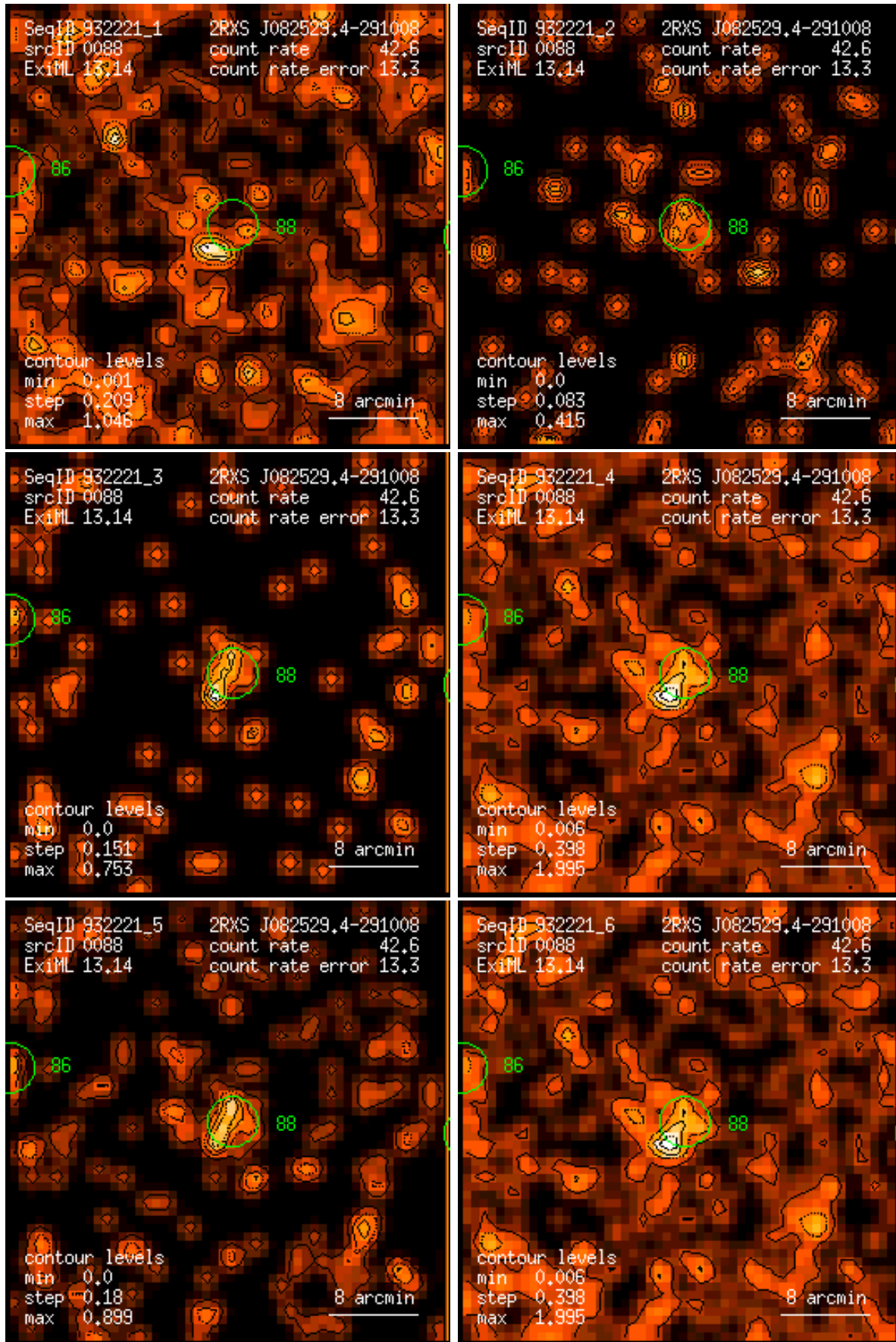
Figure 88: RASS 932221: detection 0088: band rate images, Gaussian filter: (1) PSPC channels 11 – 41, (2) 52 – 90, (3) 91 – 201, (4) 11 – 235, (5) 52 – 201, (6) 11 – 201. Broad band rates in counts/ks. Band rate contour levels in counts/ks/arcmin 2 .
