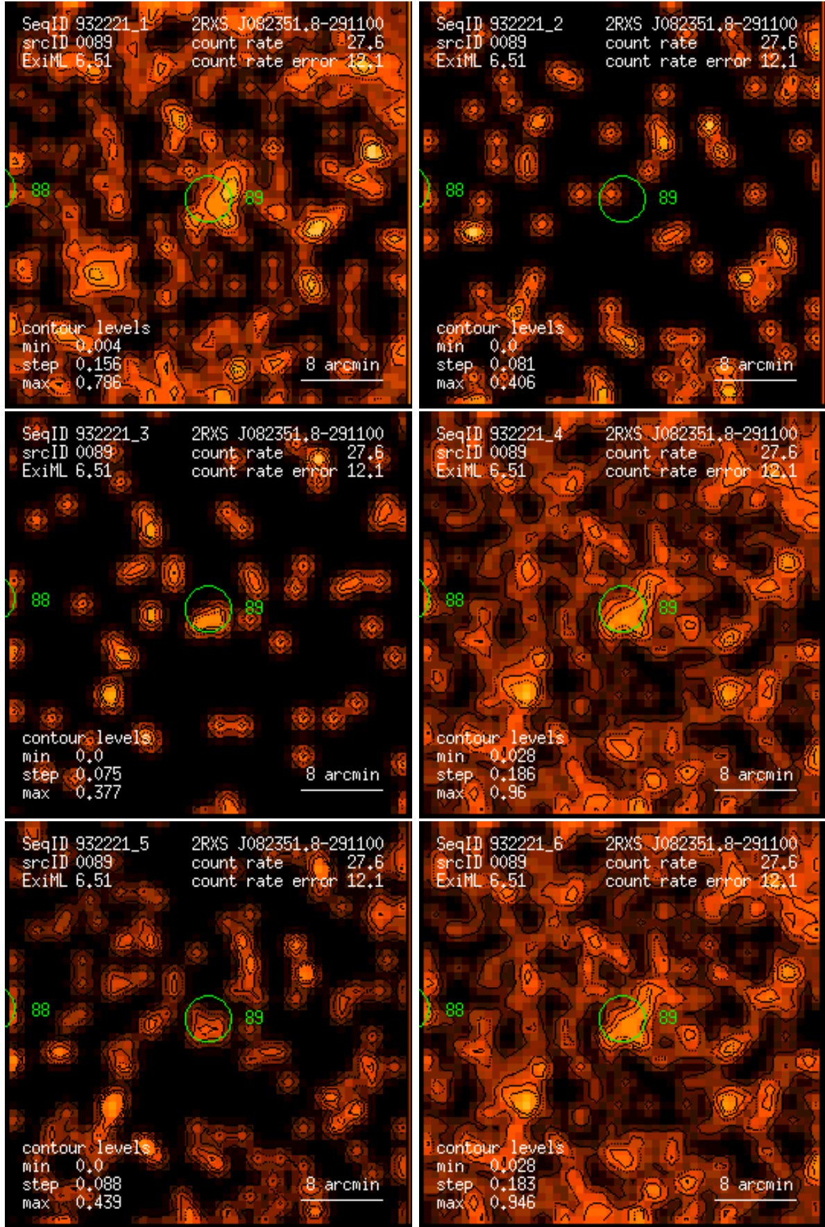
Figure 89: RASS 932221: detection 0089: band rate images, Gaussian filter: (1) PSPC channels 11 – 41, (2) 52 – 90, (3) 91 – 201, (4) 11 – 235, (5) 52 – 201, (6) 11 – 201. Broad band rates in counts/ks. Band rate contour levels in counts/ks/arcmin 2 .
