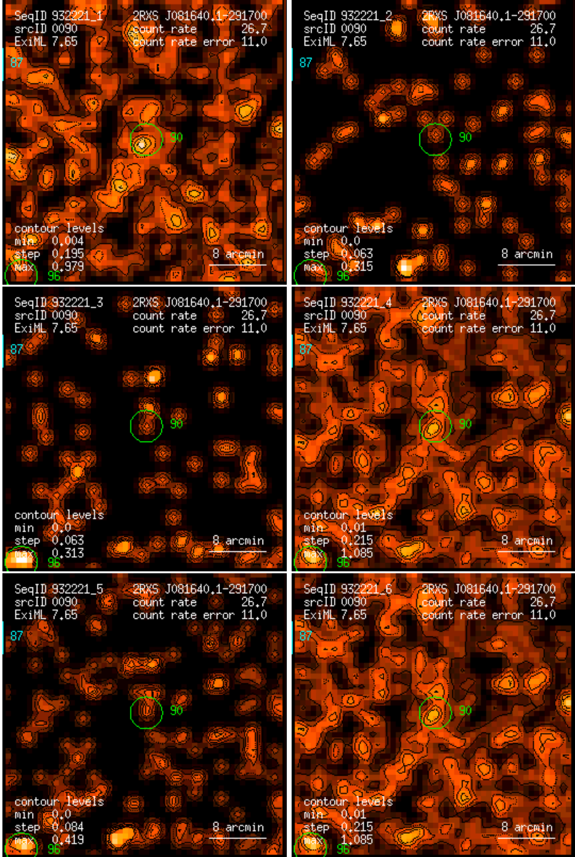
Figure 90: RASS 932221: detection 0090: band rate images, Gaussian filter: (1) PSPC channels 11 – 41, (2) 52 – 90, (3) 91 – 201, (4) 11 – 235, (5) 52 – 201, (6) 11 – 201. Broad band rates in counts/ks. Band rate contour levels in counts/ks/arcmin 2 .
