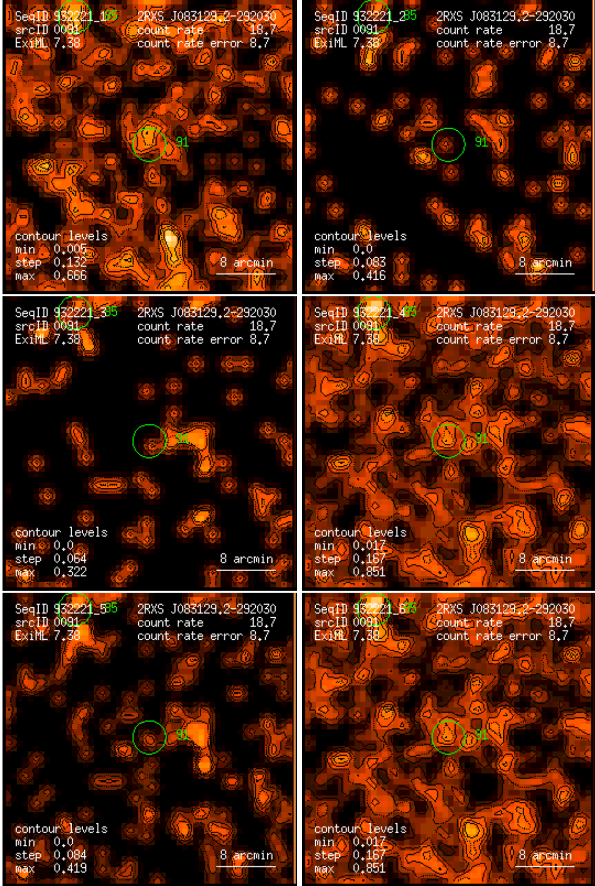
Figure 91: RASS 932221: detection 0091: band rate images, Gaussian filter: (1) PSPC channels 11 – 41, (2) 52 – 90, (3) 91 – 201, (4) 11 – 235, (5) 52 – 201, (6) 11 – 201. Broad band rates in counts/ks. Band rate contour levels in counts/ks/arcmin 2 .
