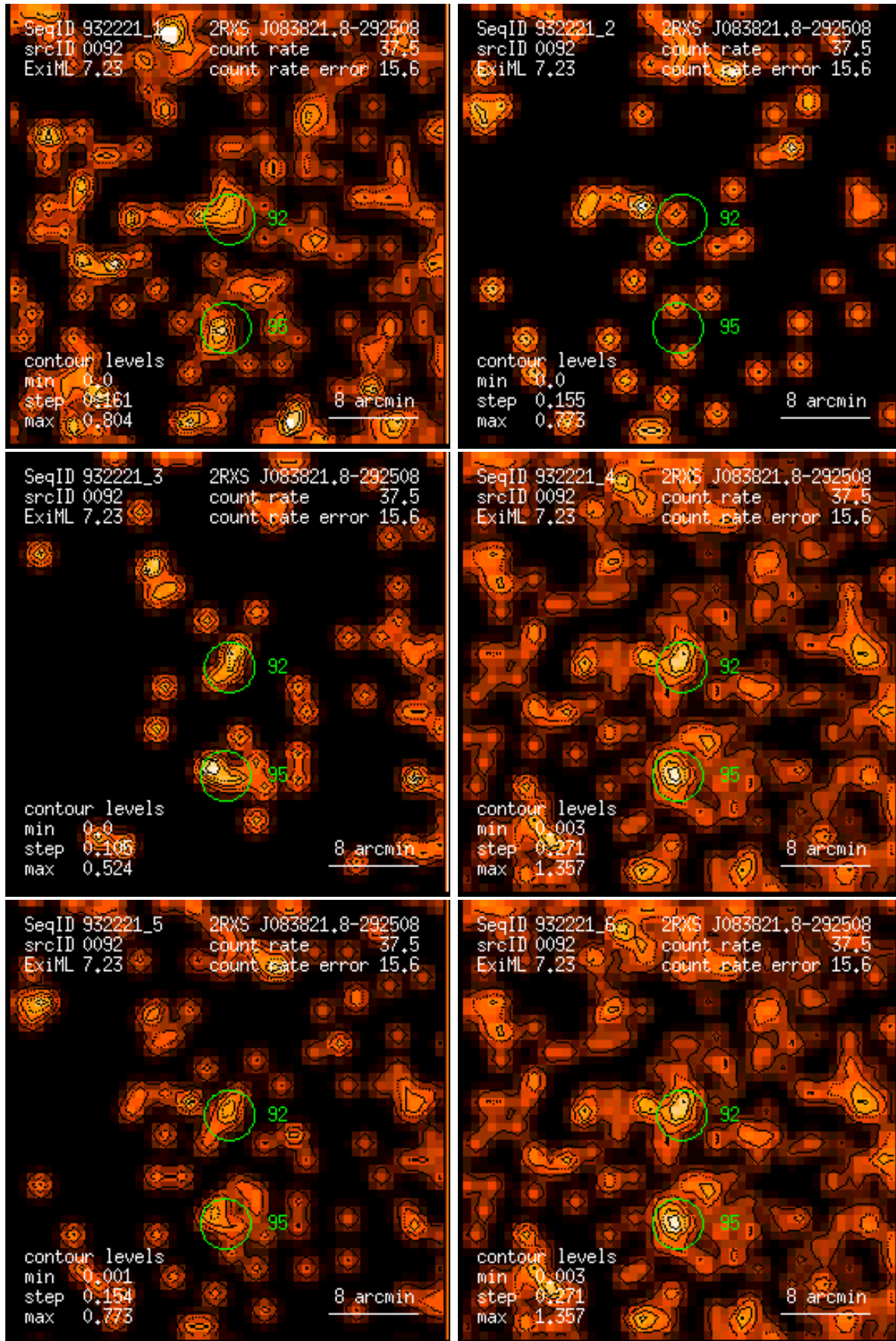
Figure 92: RASS 932221: detection 0092: band rate images, Gaussian filter: (1) PSPC channels 11 – 41, (2) 52 – 90, (3) 91 – 201, (4) 11 – 235, (5) 52 – 201, (6) 11 – 201. Broad band rates in counts/ks. Band rate contour levels in counts/ks/arcmin 2 .
