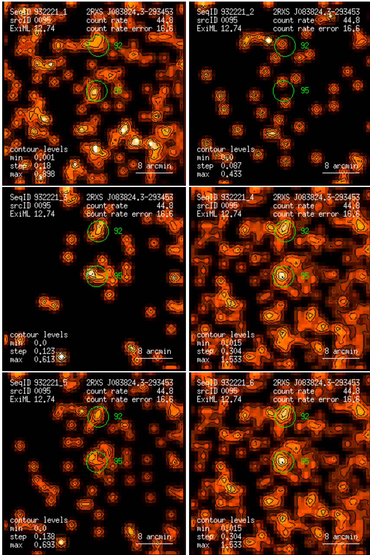
Figure 95: RASS 932221: detection 0095: band rate images, Gaussian filter: (1) PSPC channels 11 – 41, (2) 52 – 90, (3) 91 – 201, (4) 11 – 235, (5) 52 – 201, (6) 11 – 201. Broad band rates in counts/ks. Band rate contour levels in counts/ks/arcmin 2 .
