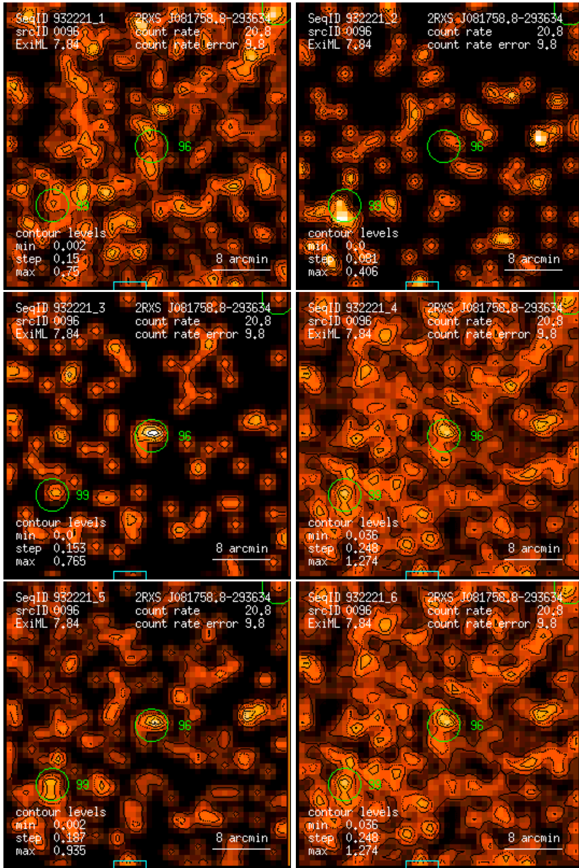
Figure 96: RASS 932221: detection 0096: band rate images, Gaussian filter: (1) PSPC channels 11 – 41, (2) 52 – 90, (3) 91 – 201, (4) 11 – 235, (5) 52 – 201, (6) 11 – 201. Broad band rates in counts/ks. Band rate contour levels in counts/ks/arcmin 2 .
