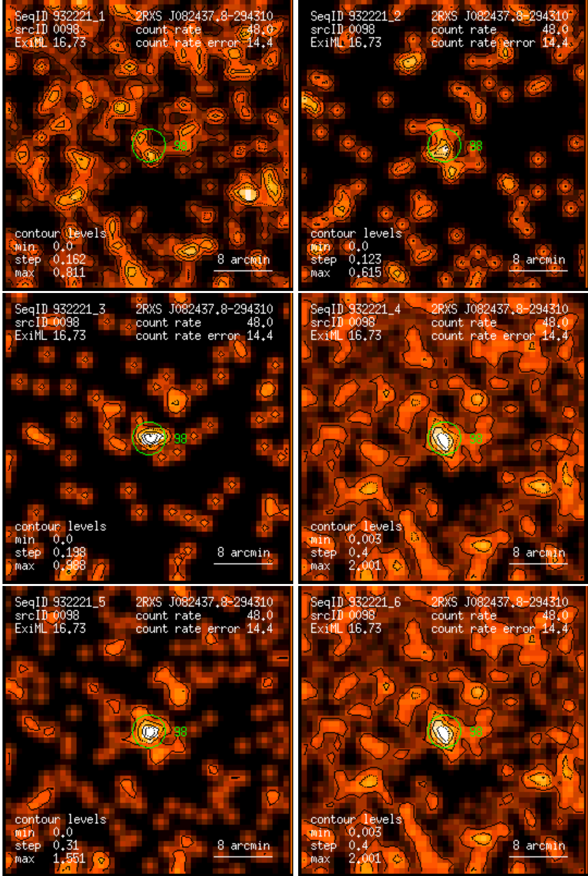
Figure 98: RASS 932221: detection 0098: band rate images, Gaussian filter: (1) PSPC channels 11 – 41, (2) 52 – 90, (3) 91 – 201, (4) 11 – 235, (5) 52 – 201, (6) 11 – 201. Broad band rates in counts/ks. Band rate contour levels in counts/ks/arcmin 2 .
