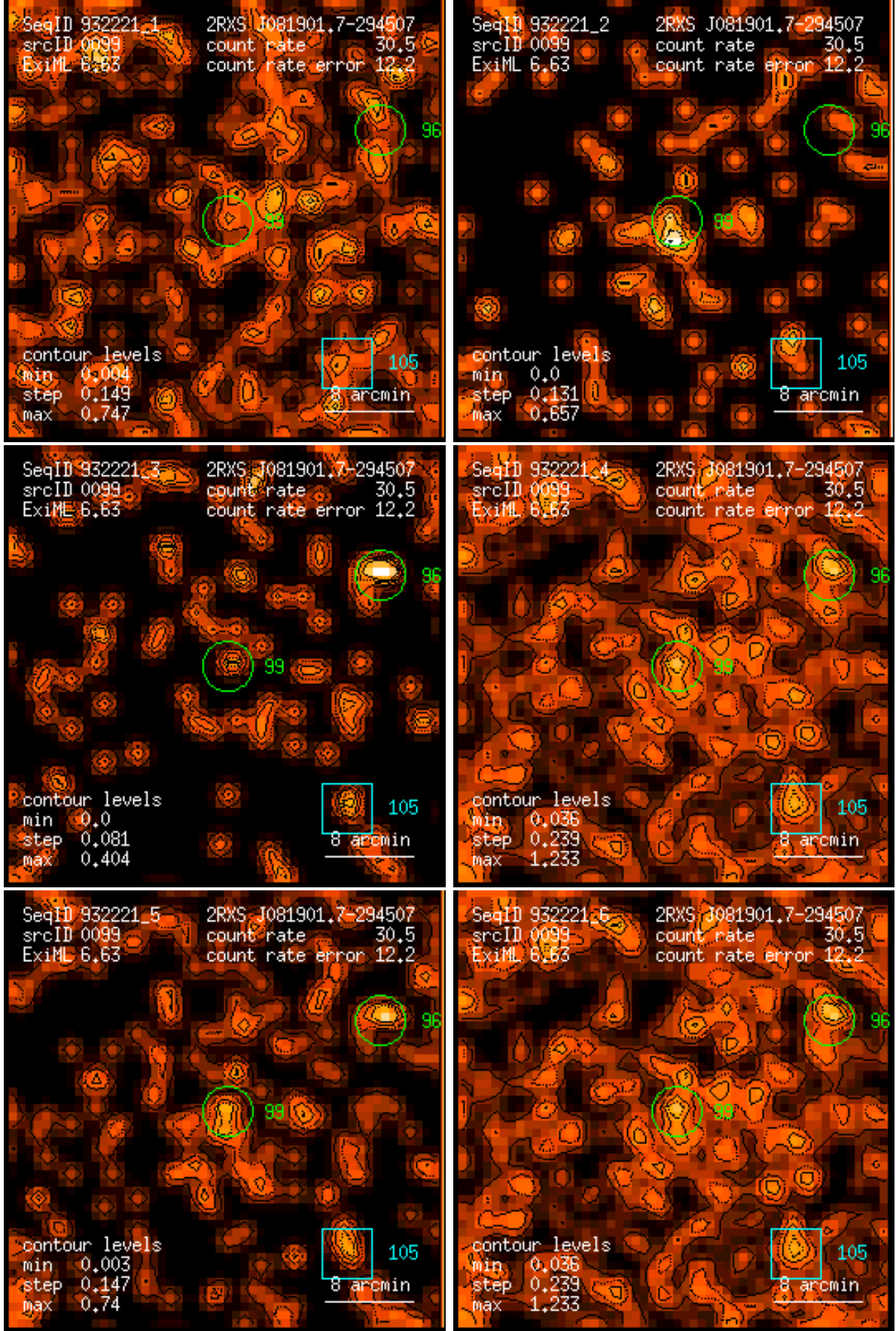
Figure 99: RASS 932221: detection 0099: band rate images, Gaussian filter: (1) PSPC channels 11 – 41, (2) 52 – 90, (3) 91 – 201, (4) 11 – 235, (5) 52 – 201, (6) 11 – 201. Broad band rates in counts/ks. Band rate contour levels in counts/ks/arcmin 2 .
