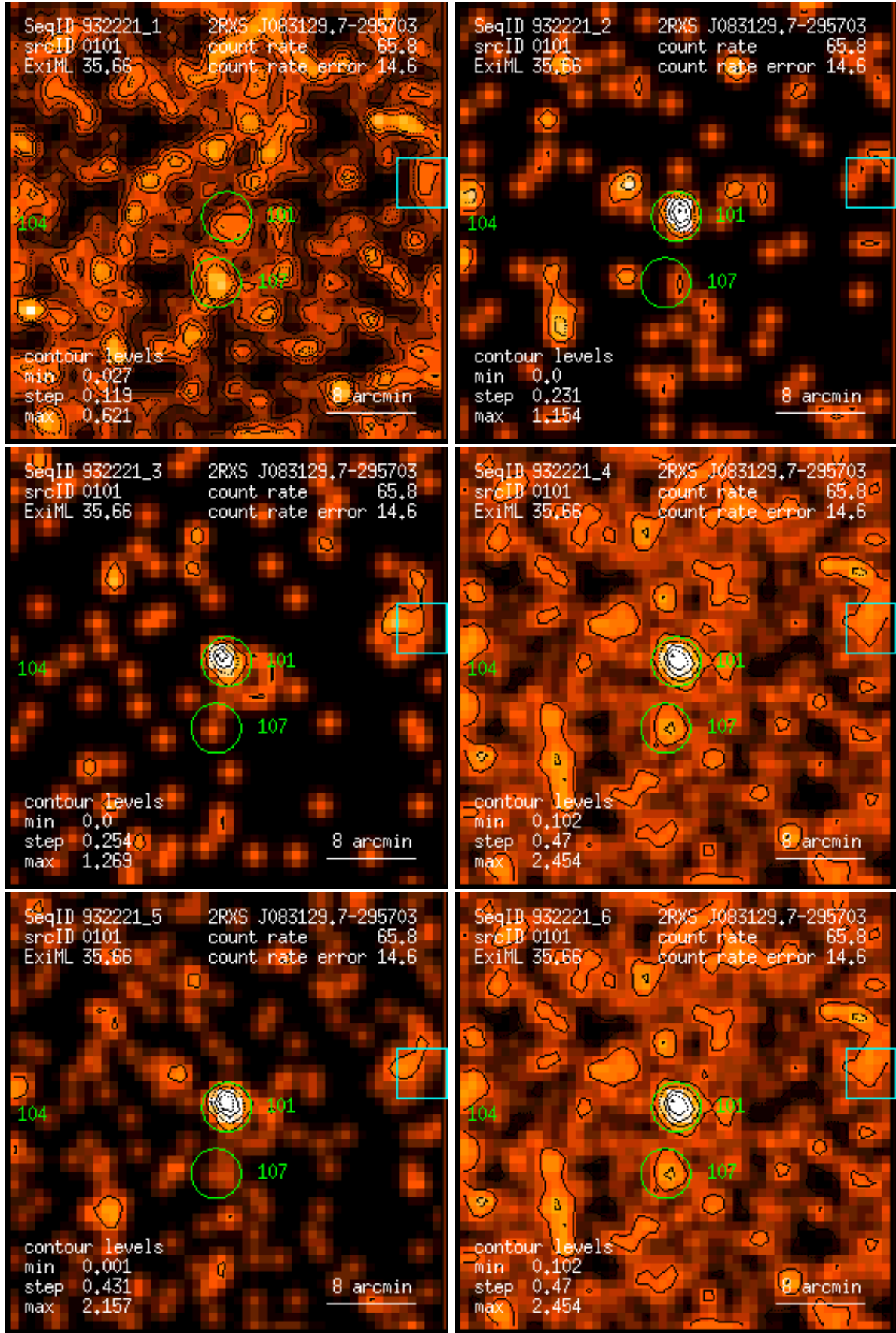
Figure 101: RASS 932221: detection 0101: band rate images, Gaussian filter: (1) PSPC channels 11 – 41, (2) 52 – 90, (3) 91 – 201, (4) 11 – 235, (5) 52 – 201, (6) 11 – 201. Broad band rates in counts/ks. Band rate contour levels in counts/ks/arcmin 2 .
