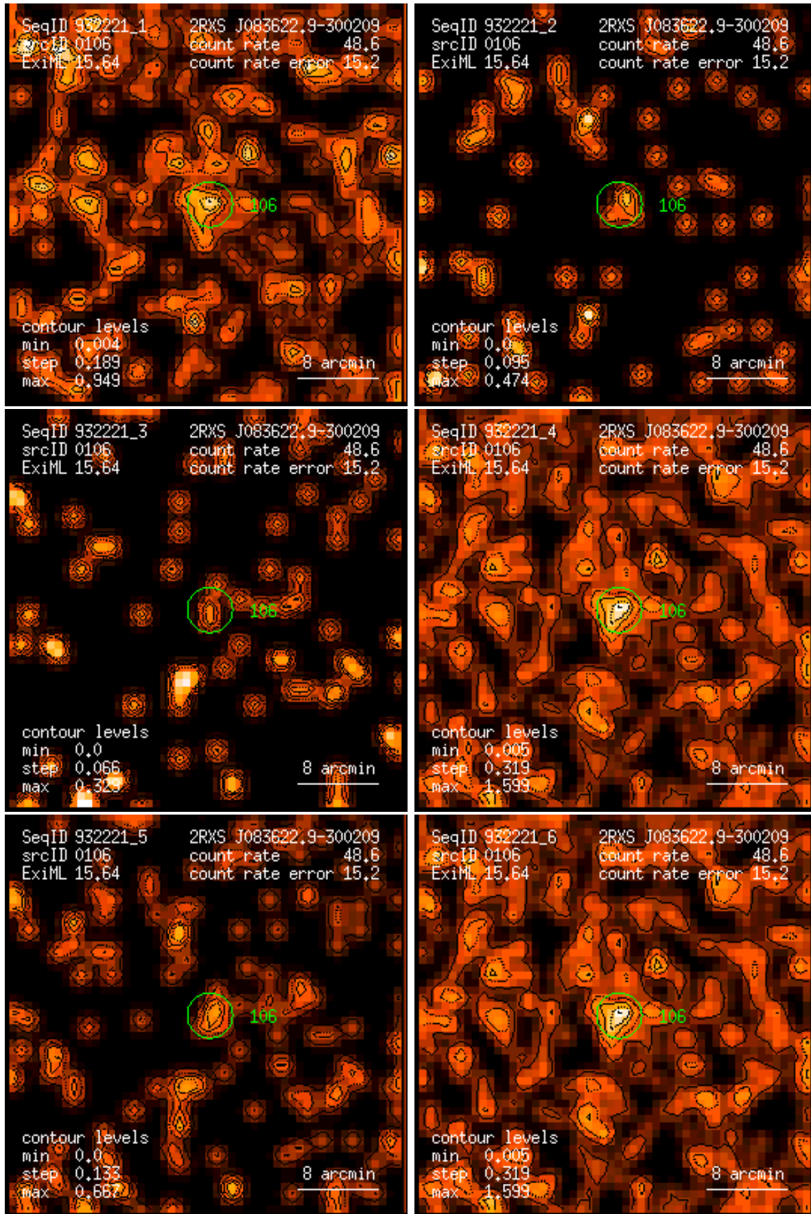
Figure 106: RASS 932221: detection 0106: band rate images, Gaussian filter: (1) PSPC channels 11 – 41, (2) 52 – 90, (3) 91 – 201, (4) 11 – 235, (5) 52 – 201, (6) 11 – 201. Broad band rates in counts/ks. Band rate contour levels in counts/ks/arcmin 2 .
