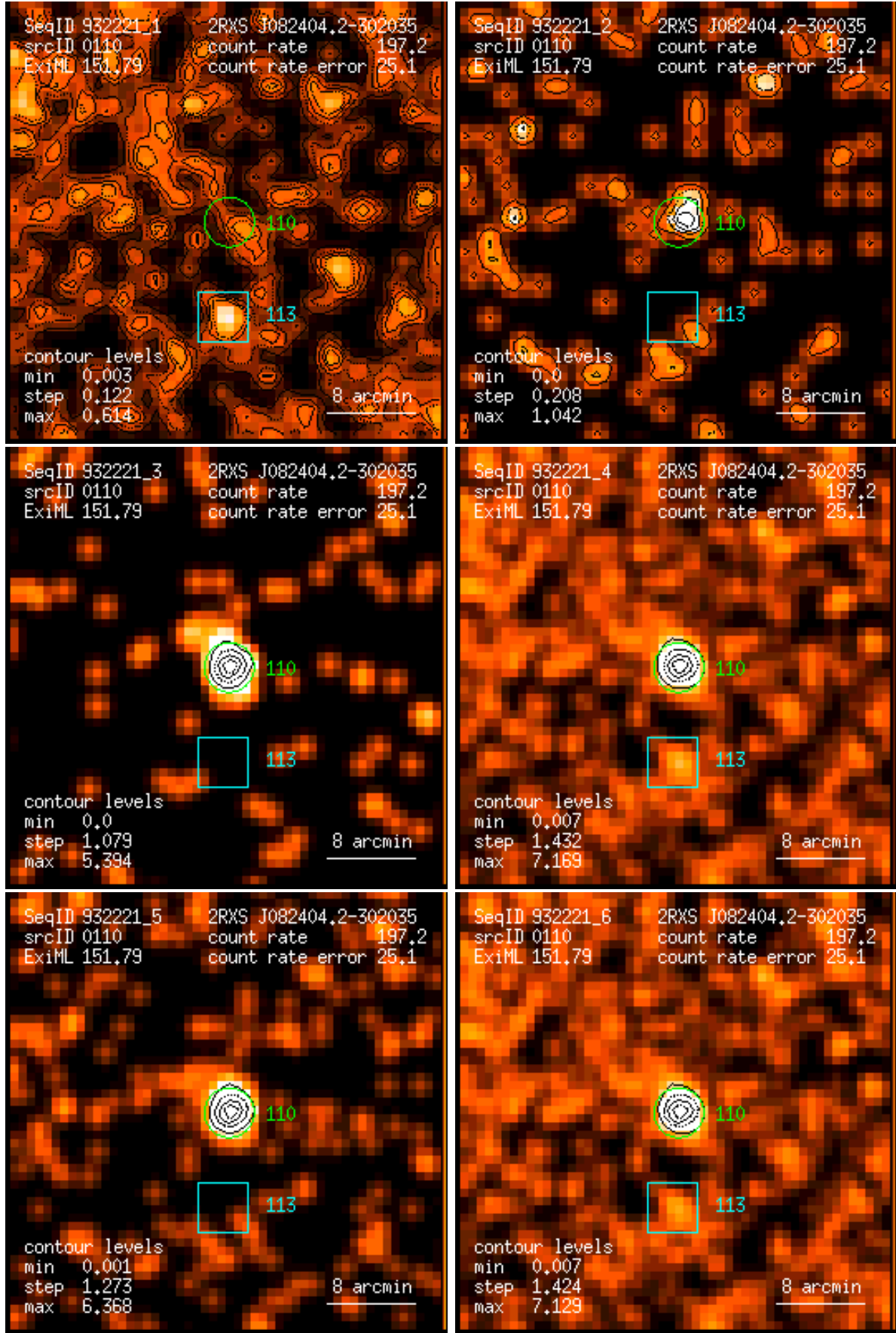
Figure 110: RASS 932221: detection 0110: band rate images, Gaussian filter: (1) PSPC channels 11 – 41, (2) 52 – 90, (3) 91 – 201, (4) 11 – 235, (5) 52 – 201, (6) 11 – 201. Broad band rates in counts/ks. Band rate contour levels in counts/ks/arcmin 2 .
