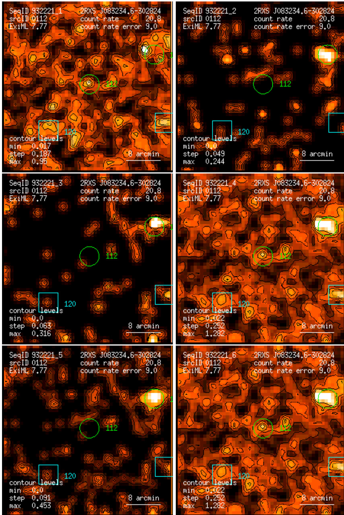
Figure 112: RASS 932221: detection 0112: band rate images, Gaussian filter: (1) PSPC channels 11 – 41, (2) 52 – 90, (3) 91 – 201, (4) 11 – 235, (5) 52 – 201, (6) 11 – 201. Broad band rates in counts/ks. Band rate contour levels in counts/ks/arcmin 2 .
