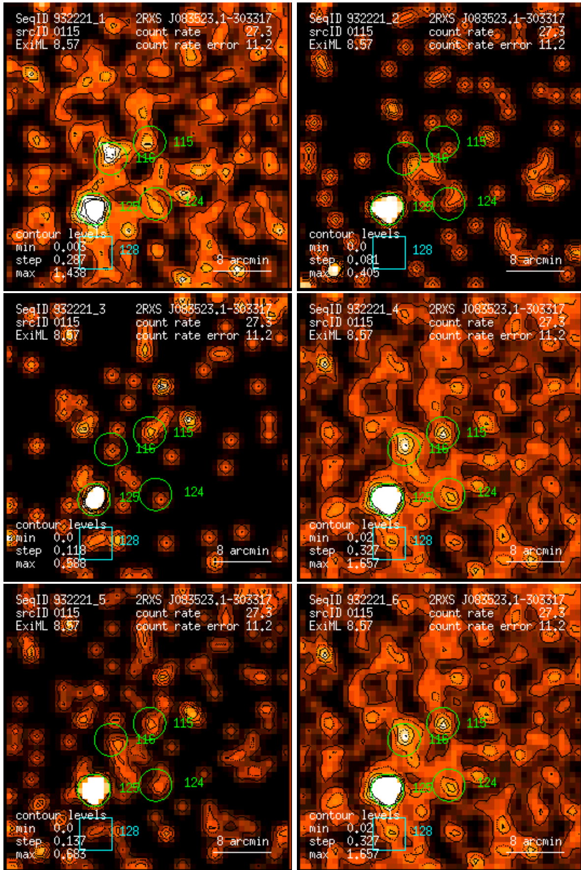
Figure 115: RASS 932221: detection 0115: band rate images, Gaussian filter: (1) PSPC channels 11 – 41, (2) 52 – 90, (3) 91 – 201, (4) 11 – 235, (5) 52 – 201, (6) 11 – 201. Broad band rates in counts/ks. Band rate contour levels in counts/ks/arcmin 2 .
