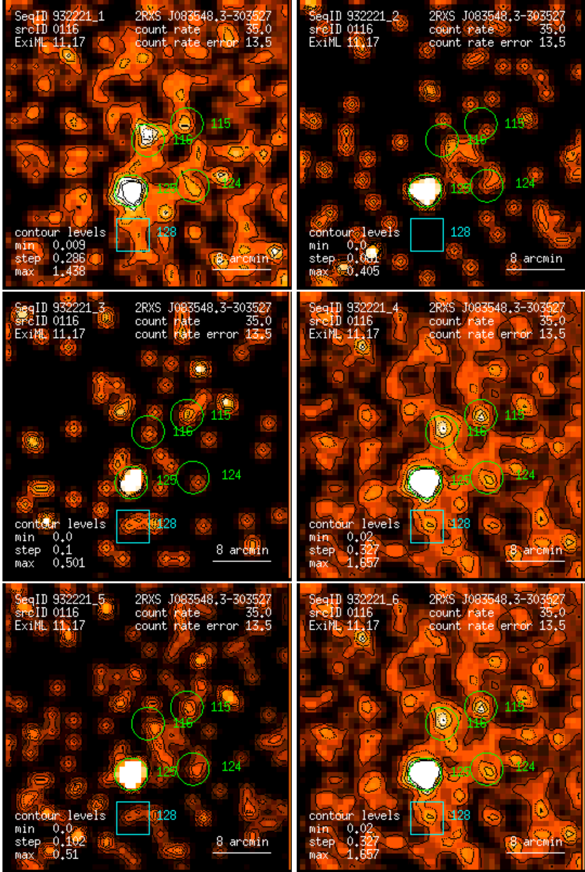
Figure 116: RASS 932221: detection 0116: band rate images, Gaussian filter: (1) PSPC channels 11 – 41, (2) 52 – 90, (3) 91 – 201, (4) 11 – 235, (5) 52 – 201, (6) 11 – 201. Broad band rates in counts/ks. Band rate contour levels in counts/ks/arcmin 2 .
