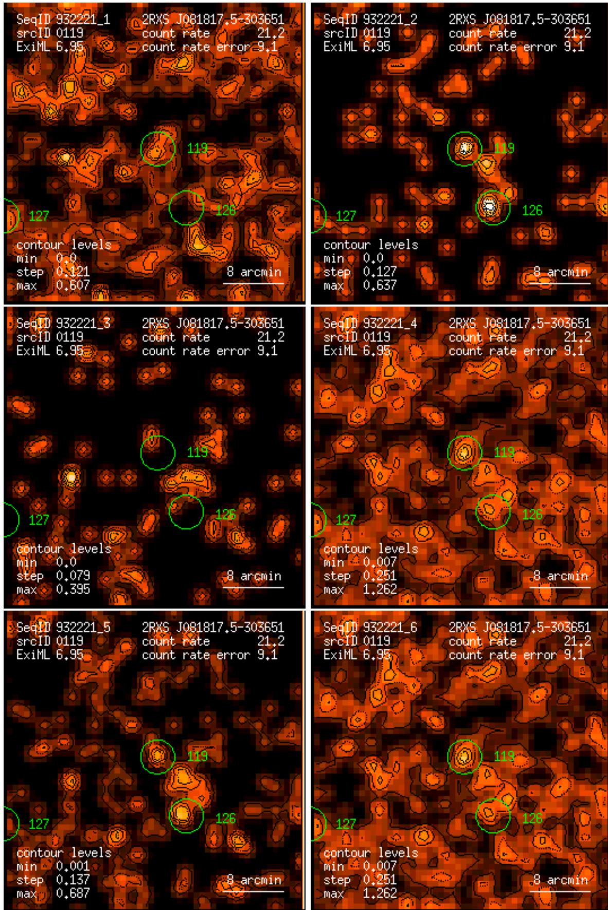
Figure 119: RASS 932221: detection 0119: band rate images, Gaussian filter: (1) PSPC channels 11 – 41, (2) 52 – 90, (3) 91 – 201, (4) 11 – 235, (5) 52 – 201, (6) 11 – 201. Broad band rates in counts/ks. Band rate contour levels in counts/ks/arcmin 2 .
