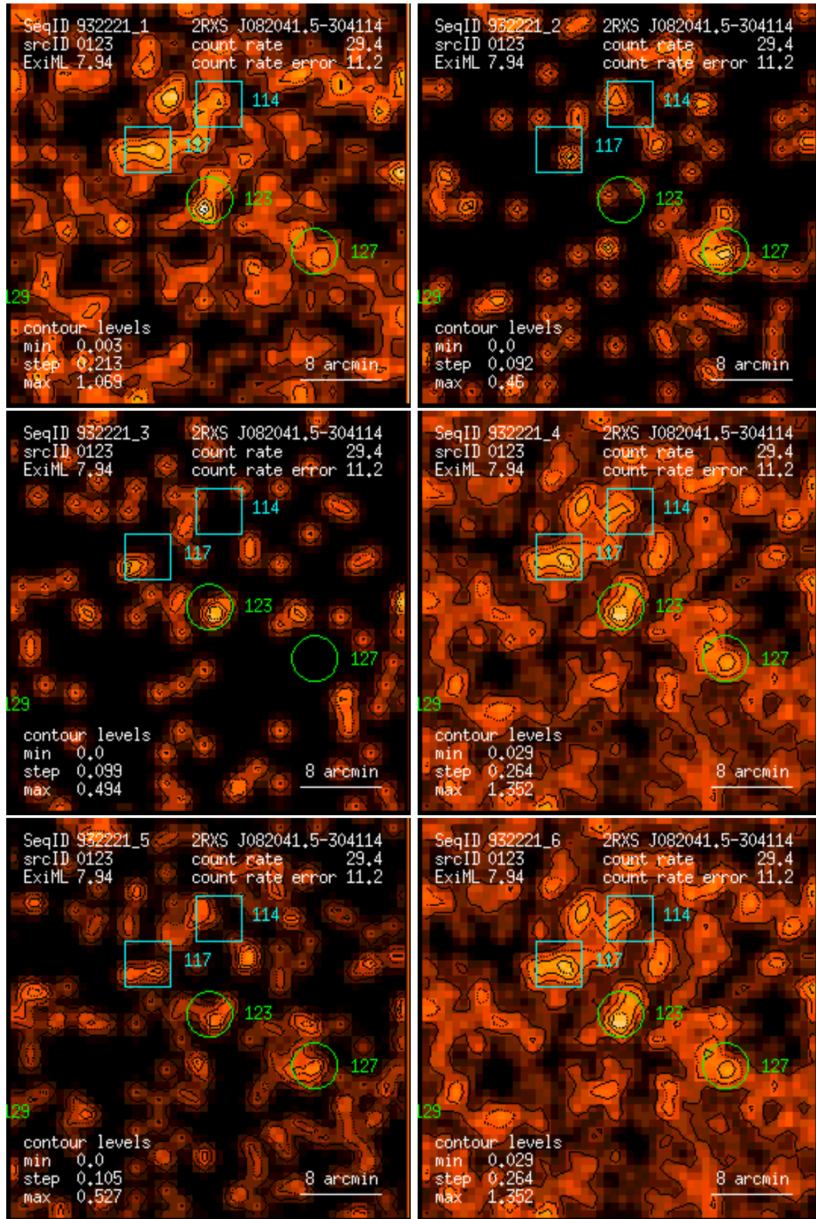
Figure 123: RASS 932221: detection 0123: band rate images, Gaussian filter: (1) PSPC channels 11 – 41, (2) 52 – 90, (3) 91 – 201, (4) 11 – 235, (5) 52 – 201, (6) 11 – 201. Broad band rates in counts/ks. Band rate contour levels in counts/ks/arcmin 2 .
