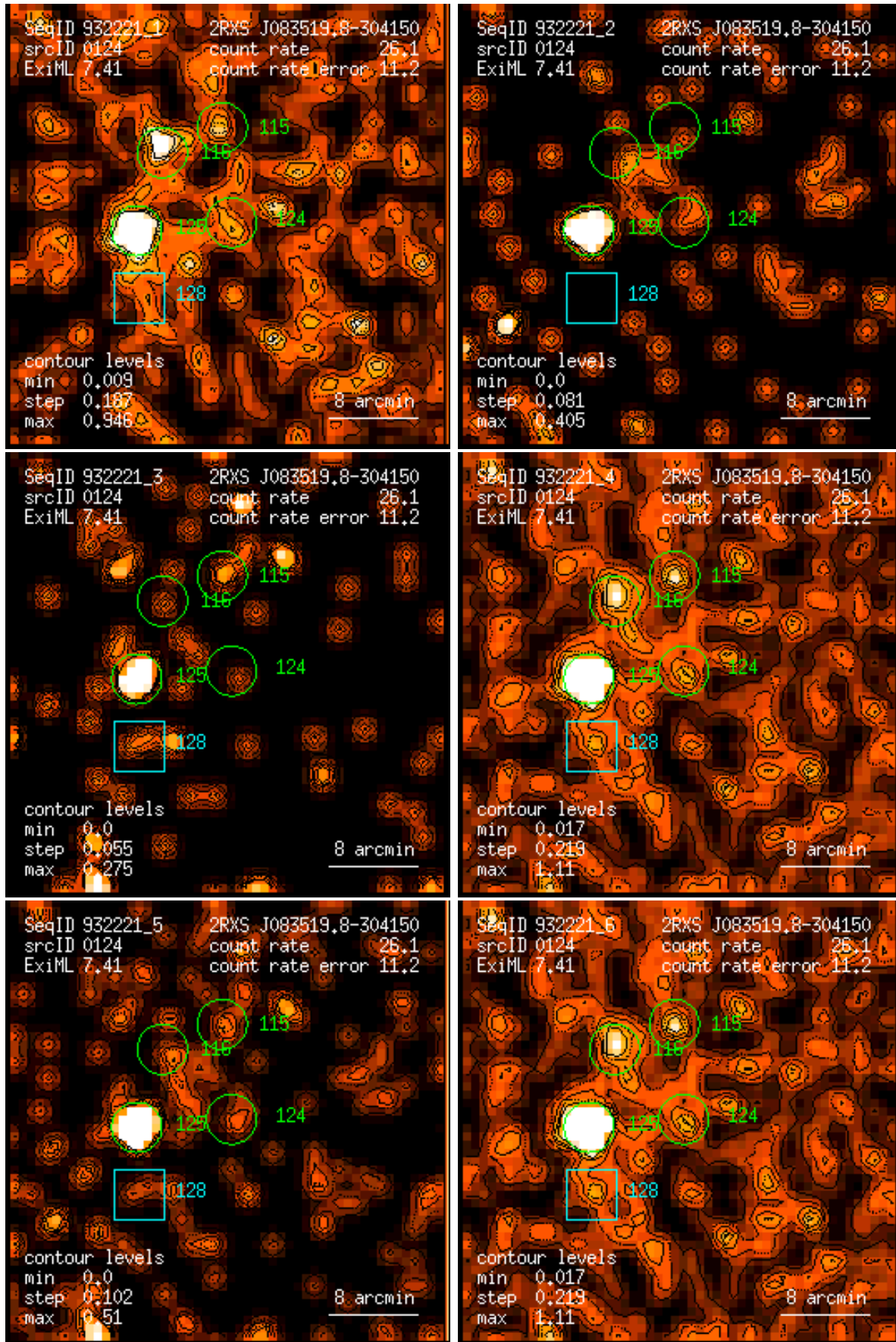
Figure 124: RASS 932221: detection 0124: band rate images, Gaussian filter: (1) PSPC channels 11 – 41, (2) 52 – 90, (3) 91 – 201, (4) 11 – 235, (5) 52 – 201, (6) 11 – 201. Broad band rates in counts/ks. Band rate contour levels in counts/ks/arcmin 2 .
