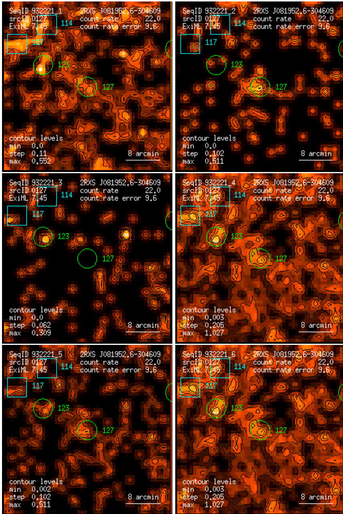
Figure 127: RASS 932221: detection 0127: band rate images, Gaussian filter: (1) PSPC channels 11 – 41, (2) 52 – 90, (3) 91 – 201, (4) 11 – 235, (5) 52 – 201, (6) 11 – 201. Broad band rates in counts/ks. Band rate contour levels in counts/ks/arcmin 2 .
