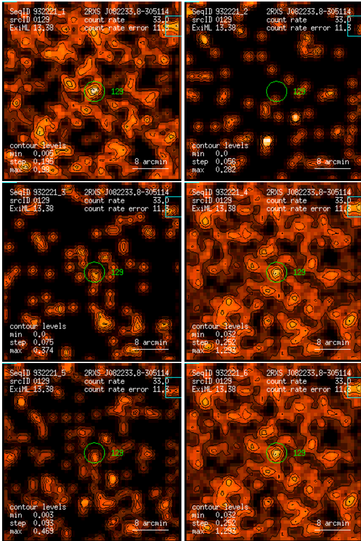
Figure 129: RASS 932221: detection 0129: band rate images, Gaussian filter: (1) PSPC channels 11 – 41, (2) 52 – 90, (3) 91 – 201, (4) 11 – 235, (5) 52 – 201, (6) 11 – 201. Broad band rates in counts/ks. Band rate contour levels in counts/ks/arcmin 2 .
