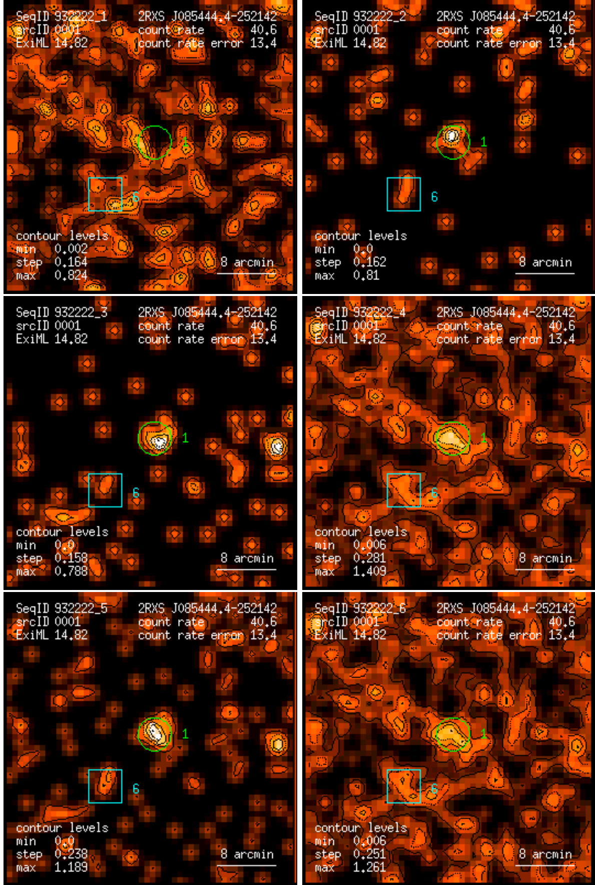
Figure 1: RASS 932222: detection 0001: band rate images, Gaussian filter: (1) PSPC channels 11 – 41, (2) 52 – 90, (3) 91 – 201, (4) 11 – 235, (5) 52 – 201, (6) 11 – 201. Broad band rates in counts/ks. Band rate contour levels in counts/ks/arcmin 2 .
