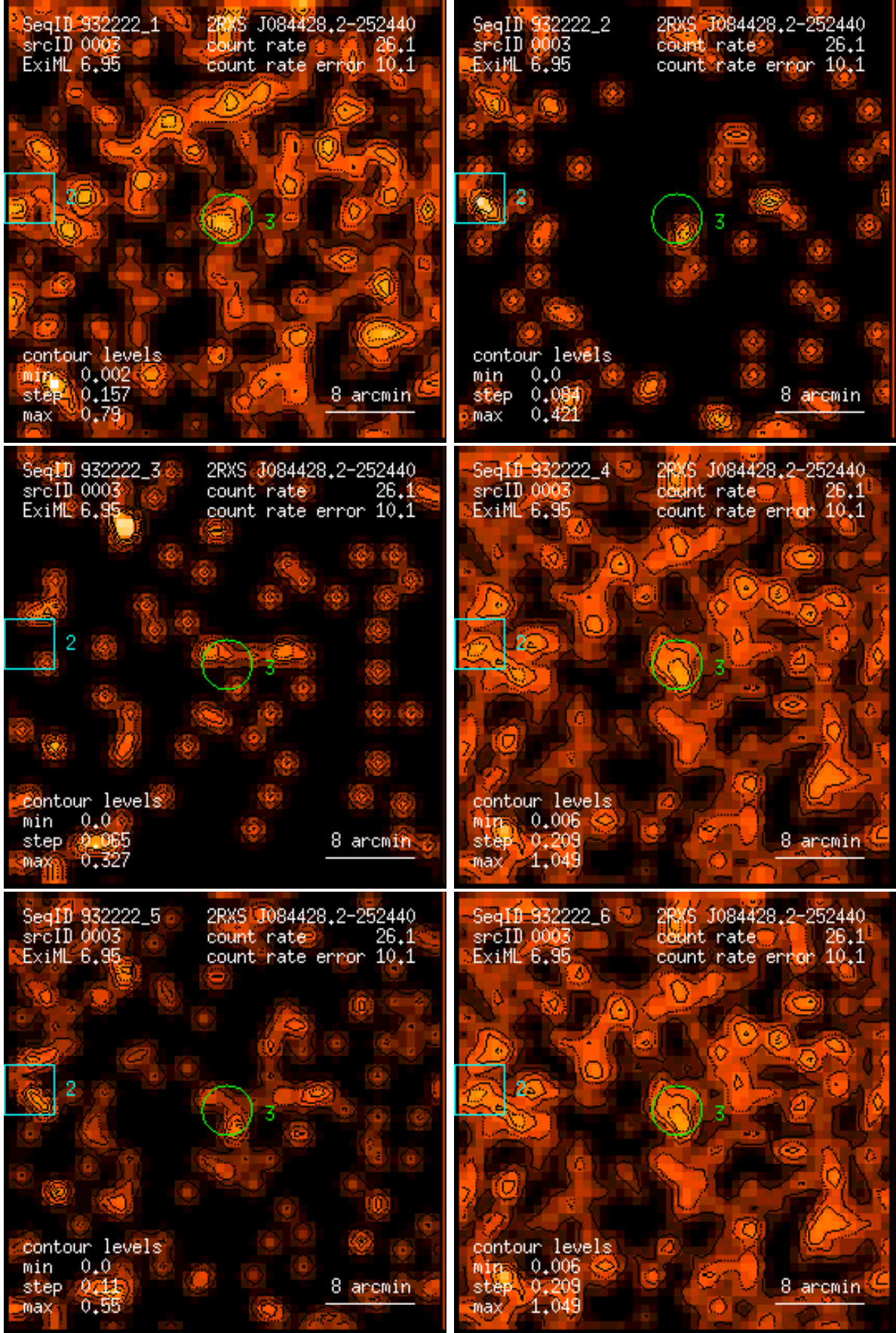
Figure 3: RASS 932222: detection 0003: band rate images, Gaussian filter: (1) PSPC channels 11 – 41, (2) 52 – 90, (3) 91 – 201, (4) 11 – 235, (5) 52 – 201, (6) 11 – 201. Broad band rates in counts/ks. Band rate contour levels in counts/ks/arcmin 2 .
