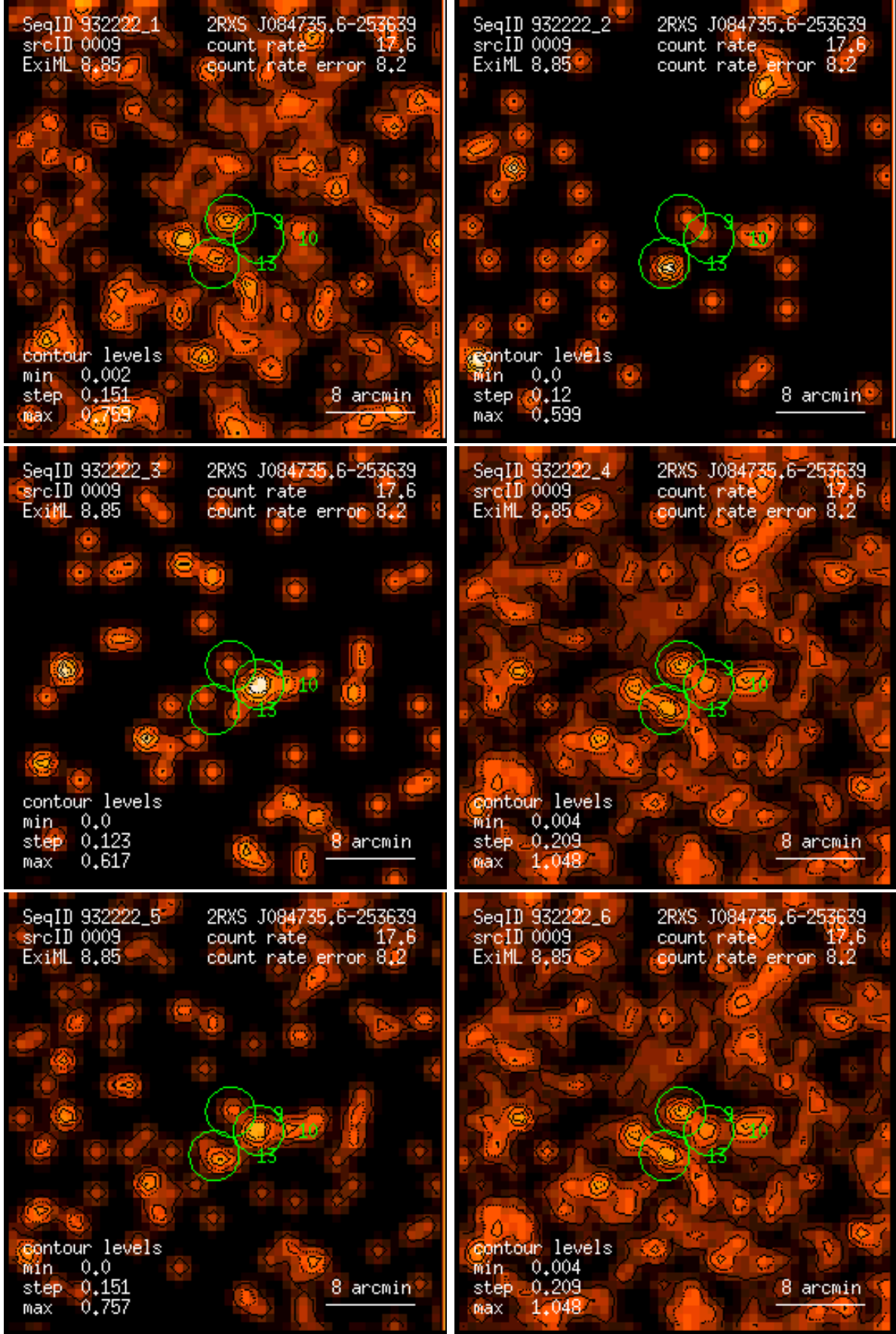
Figure 9: RASS 932222: detection 0009: band rate images, Gaussian filter: (1) PSPC channels 11 – 41, (2) 52 – 90, (3) 91 – 201, (4) 11 – 235, (5) 52 – 201, (6) 11 – 201. Broad band rates in counts/ks. Band rate contour levels in counts/ks/arcmin 2 .
