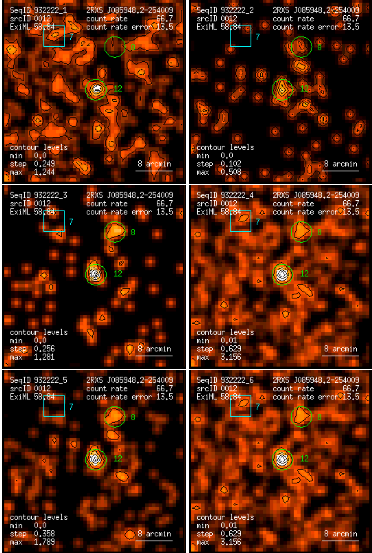
Figure 12: RASS 932222: detection 0012: band rate images, Gaussian filter: (1) PSPC channels 11 – 41, (2) 52 – 90, (3) 91 – 201, (4) 11 – 235, (5) 52 – 201, (6) 11 – 201. Broad band rates in counts/ks. Band rate contour levels in counts/ks/arcmin 2 .
