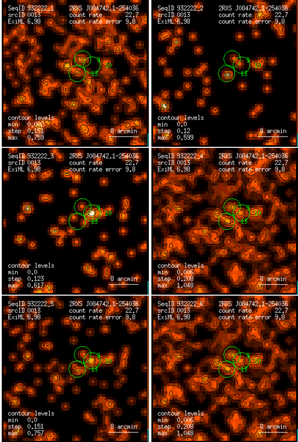
Figure 13: RASS 932222: detection 0013: band rate images, Gaussian filter: (1) PSPC channels 11 – 41, (2) 52 – 90, (3) 91 – 201, (4) 11 – 235, (5) 52 – 201, (6) 11 – 201. Broad band rates in counts/ks. Band rate contour levels in counts/ks/arcmin 2 .
