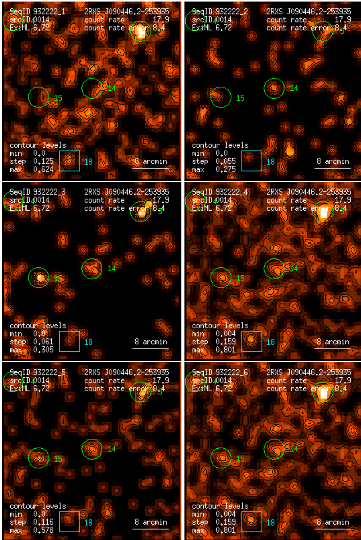
Figure 14: RASS 932222: detection 0014: band rate images, Gaussian filter: (1) PSPC channels 11 – 41, (2) 52 – 90, (3) 91 – 201, (4) 11 – 235, (5) 52 – 201, (6) 11 – 201. Broad band rates in counts/ks. Band rate contour levels in counts/ks/arcmin 2 .
