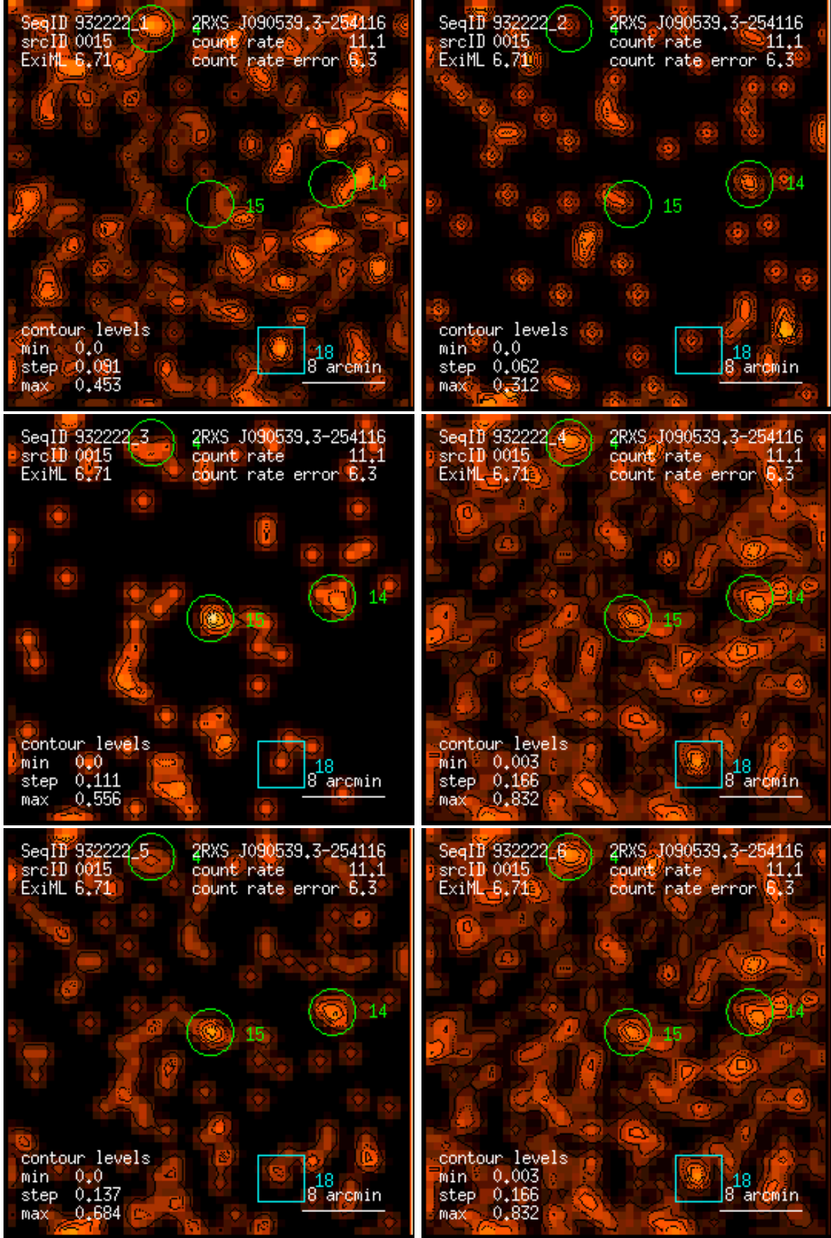
Figure 15: RASS 932222: detection 0015: band rate images, Gaussian filter: (1) PSPC channels 11 – 41, (2) 52 – 90, (3) 91 – 201, (4) 11 – 235, (5) 52 – 201, (6) 11 – 201. Broad band rates in counts/ks. Band rate contour levels in counts/ks/arcmin 2 .
