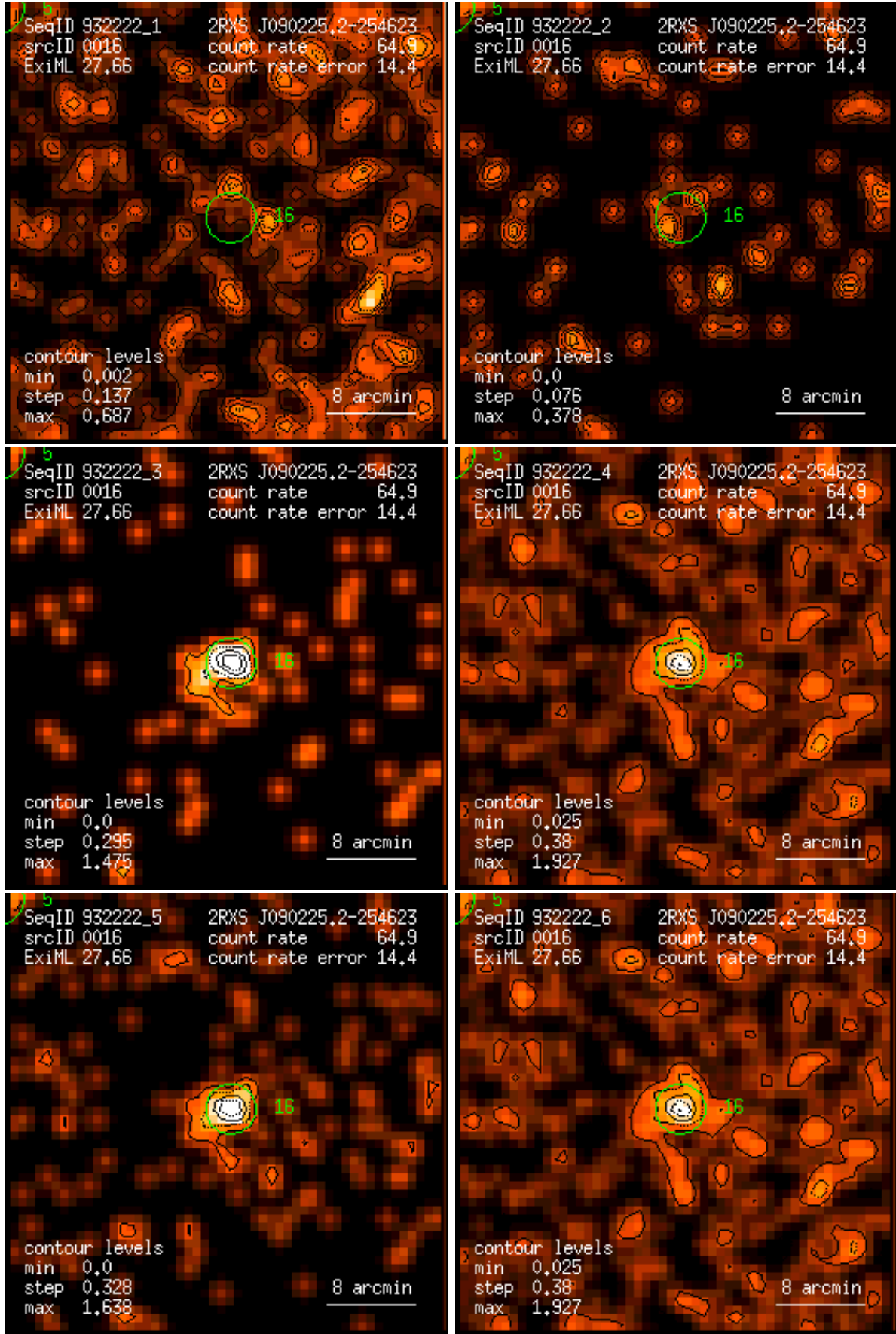
Figure 16: RASS 932222: detection 0016: band rate images, Gaussian filter: (1) PSPC channels 11 – 41, (2) 52 – 90, (3) 91 – 201, (4) 11 – 235, (5) 52 – 201, (6) 11 – 201. Broad band rates in counts/ks. Band rate contour levels in counts/ks/arcmin 2 .
