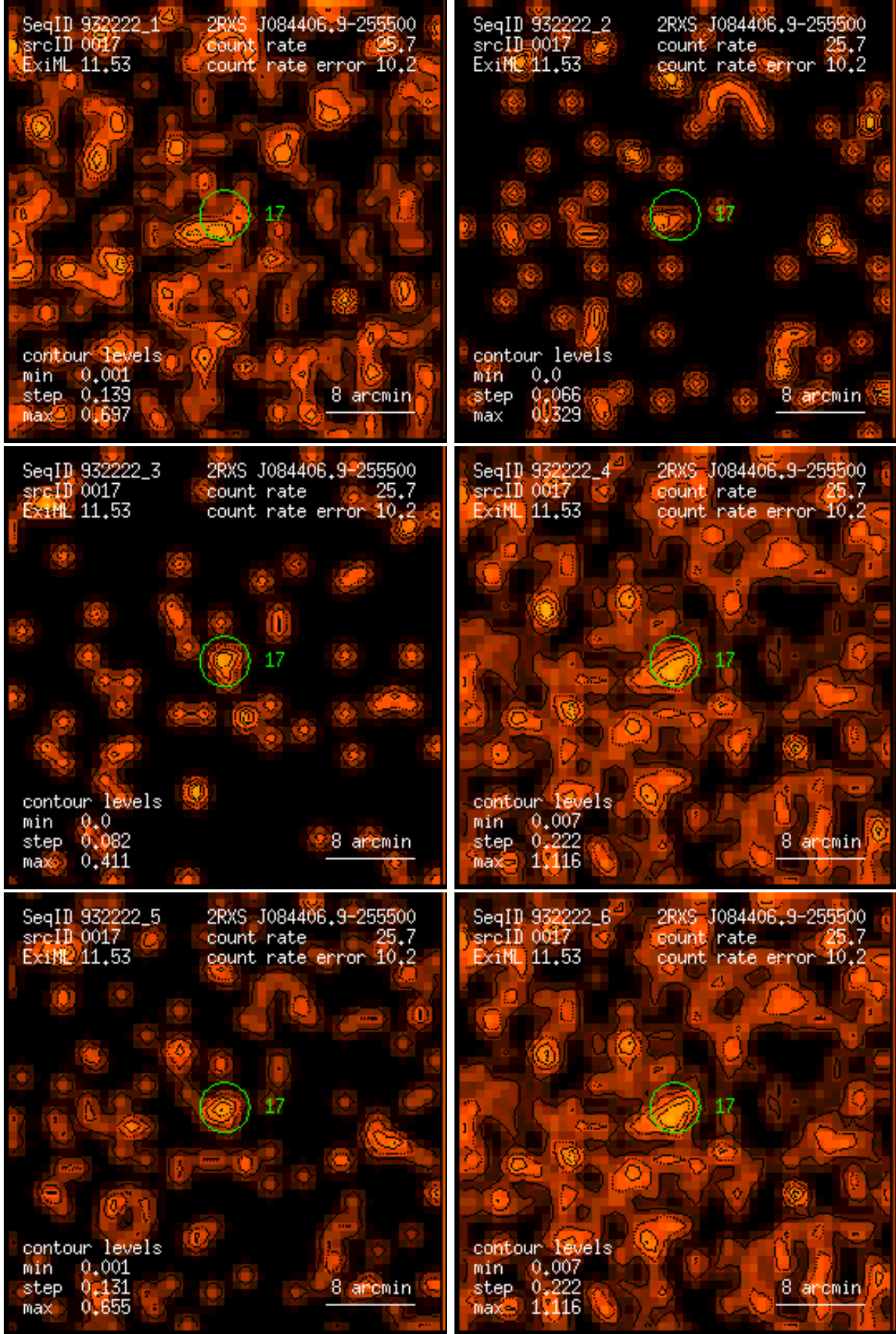
Figure 17: RASS 932222: detection 0017: band rate images, Gaussian filter: (1) PSPC channels 11 – 41, (2) 52 – 90, (3) 91 – 201, (4) 11 – 235, (5) 52 – 201, (6) 11 – 201. Broad band rates in counts/ks. Band rate contour levels in counts/ks/arcmin 2 .
