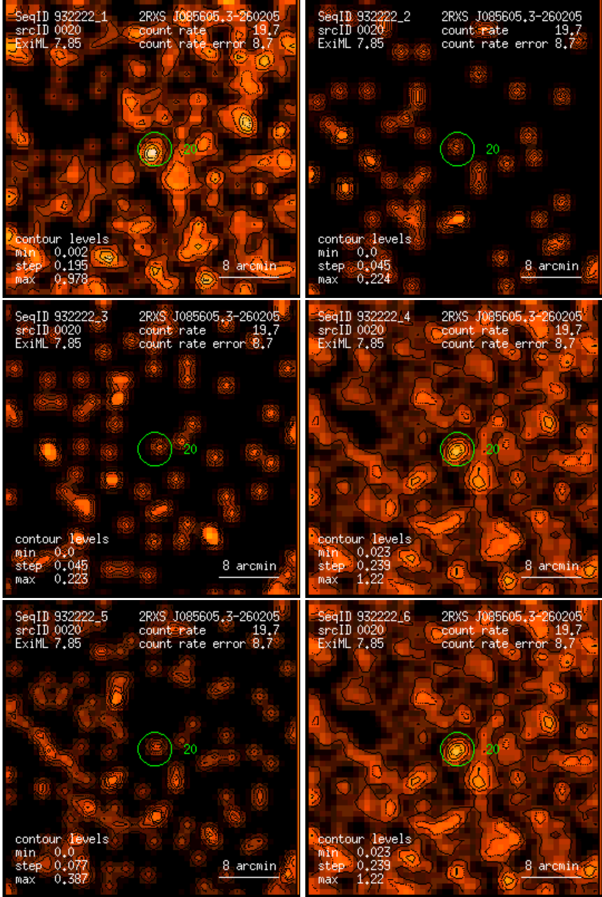
Figure 20: RASS 932222: detection 0020: band rate images, Gaussian filter: (1) PSPC channels 11 – 41, (2) 52 – 90, (3) 91 – 201, (4) 11 – 235, (5) 52 – 201, (6) 11 – 201. Broad band rates in counts/ks. Band rate contour levels in counts/ks/arcmin 2 .
